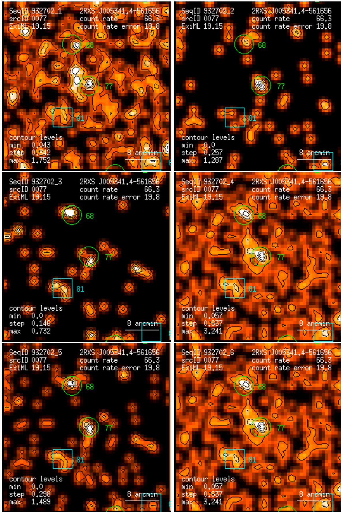
Figure 77: RASS 932702: detection 0077: band rate images, Gaussian filter: (1) PSPC channels 11 – 41, (2) 52 – 90, (3) 91 – 201, (4) 11 – 235, (5) 52 – 201, (6) 11 – 201. Broad band rates in counts/ks. Band rate contour levels in counts/ks/arcmin 2 .
