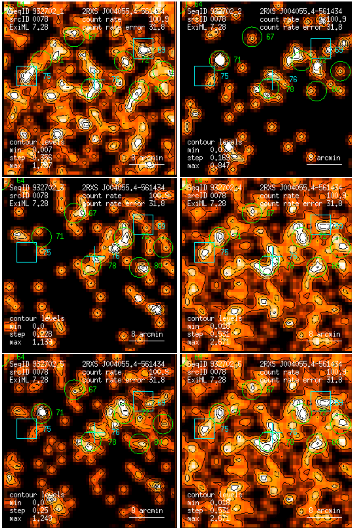
Figure 78: RASS 932702: detection 0078: band rate images, Gaussian filter: (1) PSPC channels 11 – 41, (2) 52 – 90, (3) 91 – 201, (4) 11 – 235, (5) 52 – 201, (6) 11 – 201. Broad band rates in counts/ks. Band rate contour levels in counts/ks/arcmin 2 .
