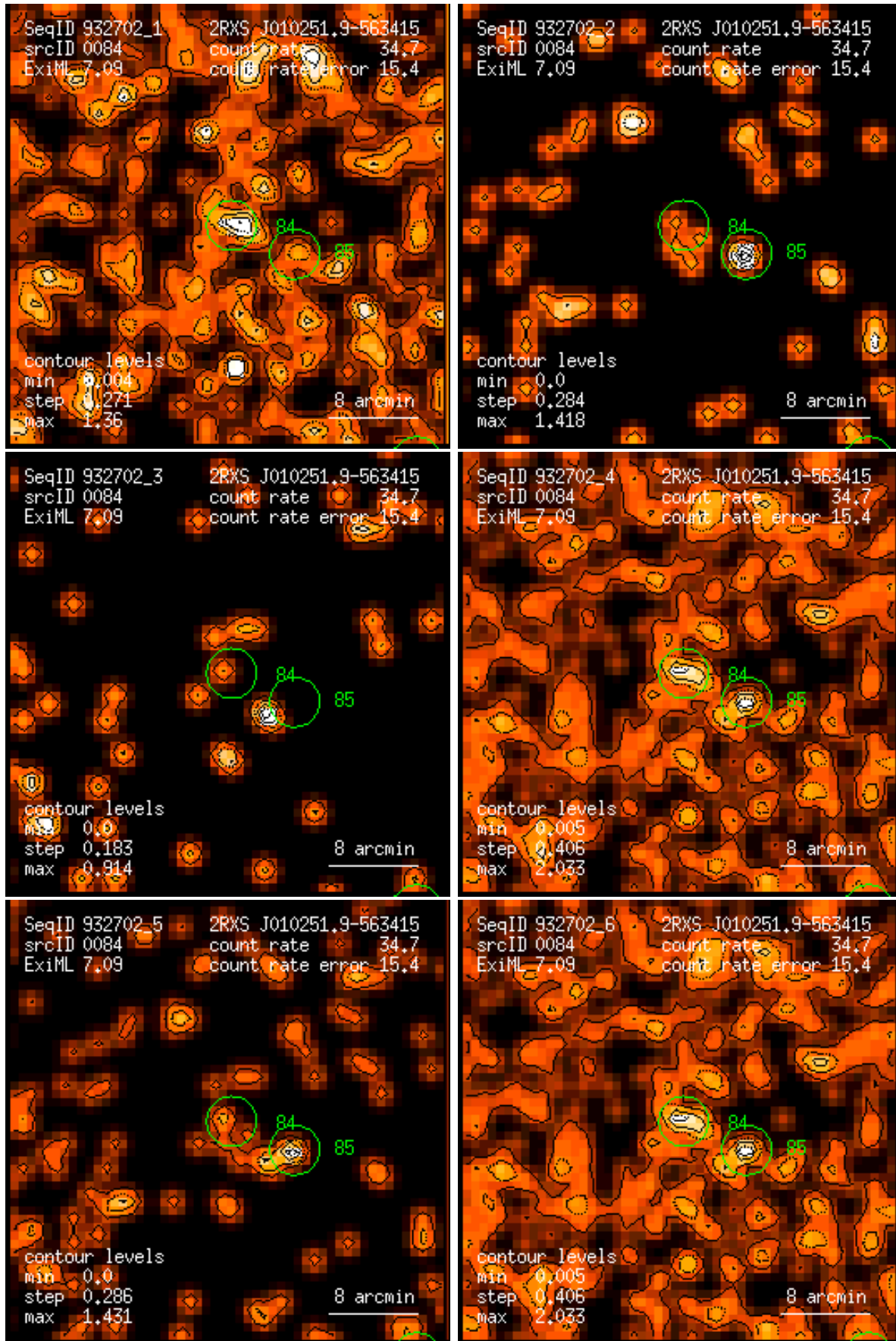
Figure 84: RASS 932702: detection 0084: band rate images, Gaussian filter: (1) PSPC channels 11 – 41, (2) 52 – 90, (3) 91 – 201, (4) 11 – 235, (5) 52 – 201, (6) 11 – 201. Broad band rates in counts/ks. Band rate contour levels in counts/ks/arcmin 2 .
