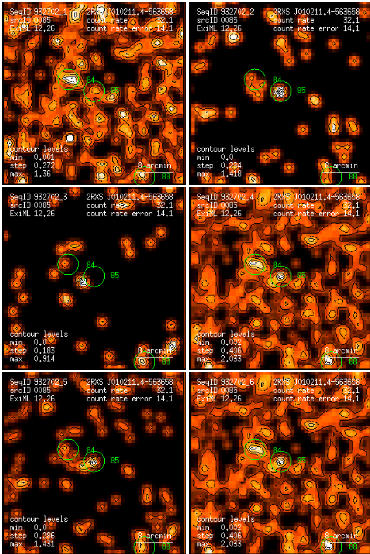
Figure 85: RASS 932702: detection 0085: band rate images, Gaussian filter: (1) PSPC channels 11 – 41, (2) 52 – 90, (3) 91 – 201, (4) 11 – 235, (5) 52 – 201, (6) 11 – 201. Broad band rates in counts/ks. Band rate contour levels in counts/ks/arcmin 2 .
