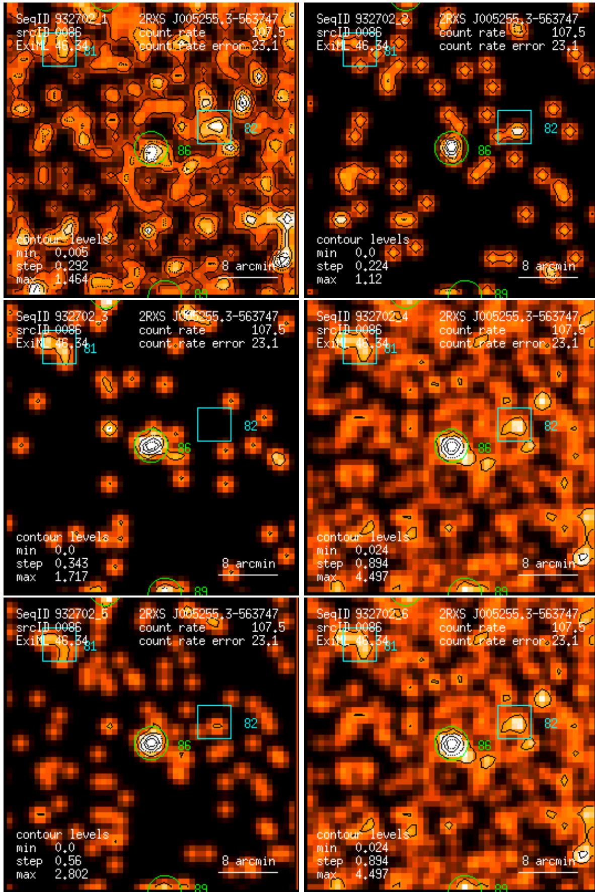
Figure 86: RASS 932702: detection 0086: band rate images, Gaussian filter: (1) PSPC channels 11 – 41, (2) 52 – 90, (3) 91 – 201, (4) 11 – 235, (5) 52 – 201, (6) 11 – 201. Broad band rates in counts/ks. Band rate contour levels in counts/ks/arcmin 2 .
