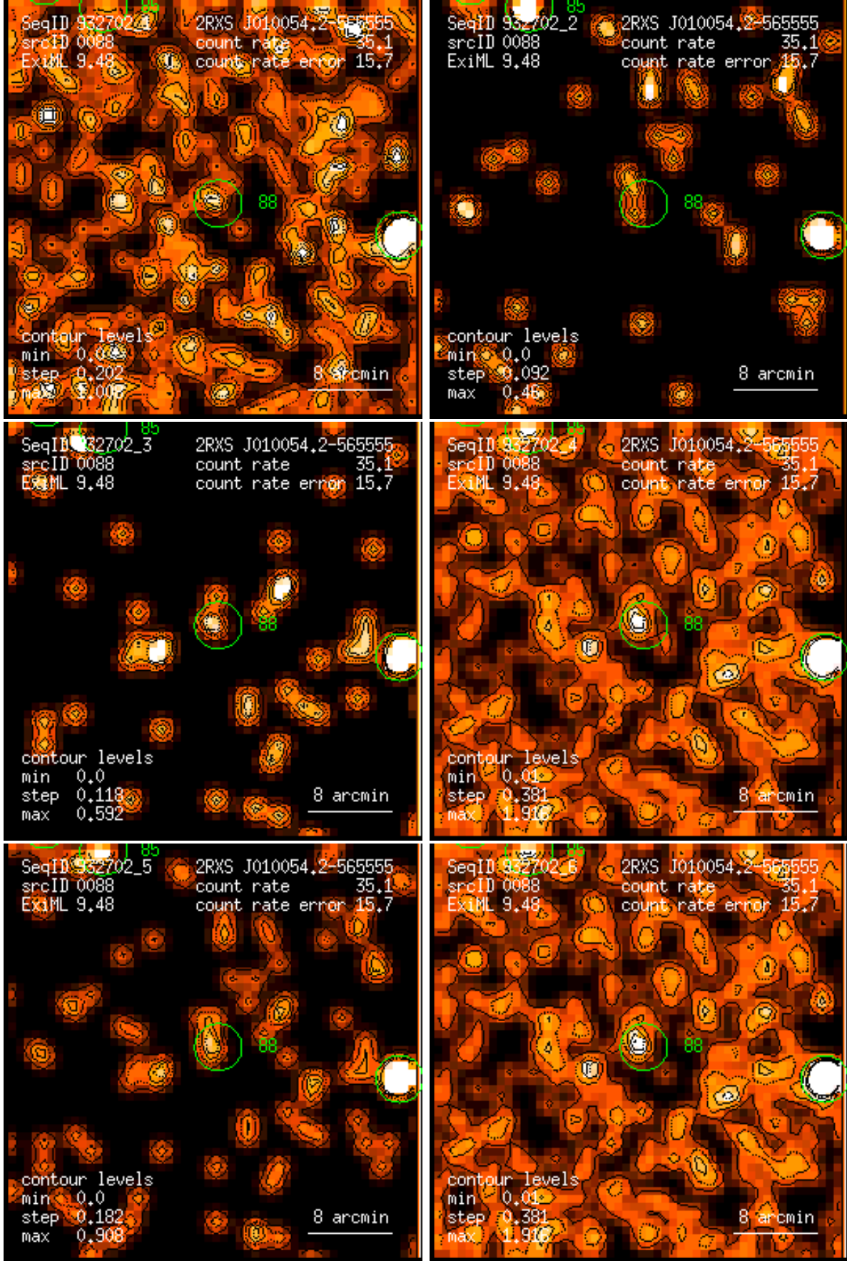
Figure 88: RASS 932702: detection 0088: band rate images, Gaussian filter: (1) PSPC channels 11 – 41, (2) 52 – 90, (3) 91 – 201, (4) 11 – 235, (5) 52 – 201, (6) 11 – 201. Broad band rates in counts/ks. Band rate contour levels in counts/ks/arcmin 2 .
