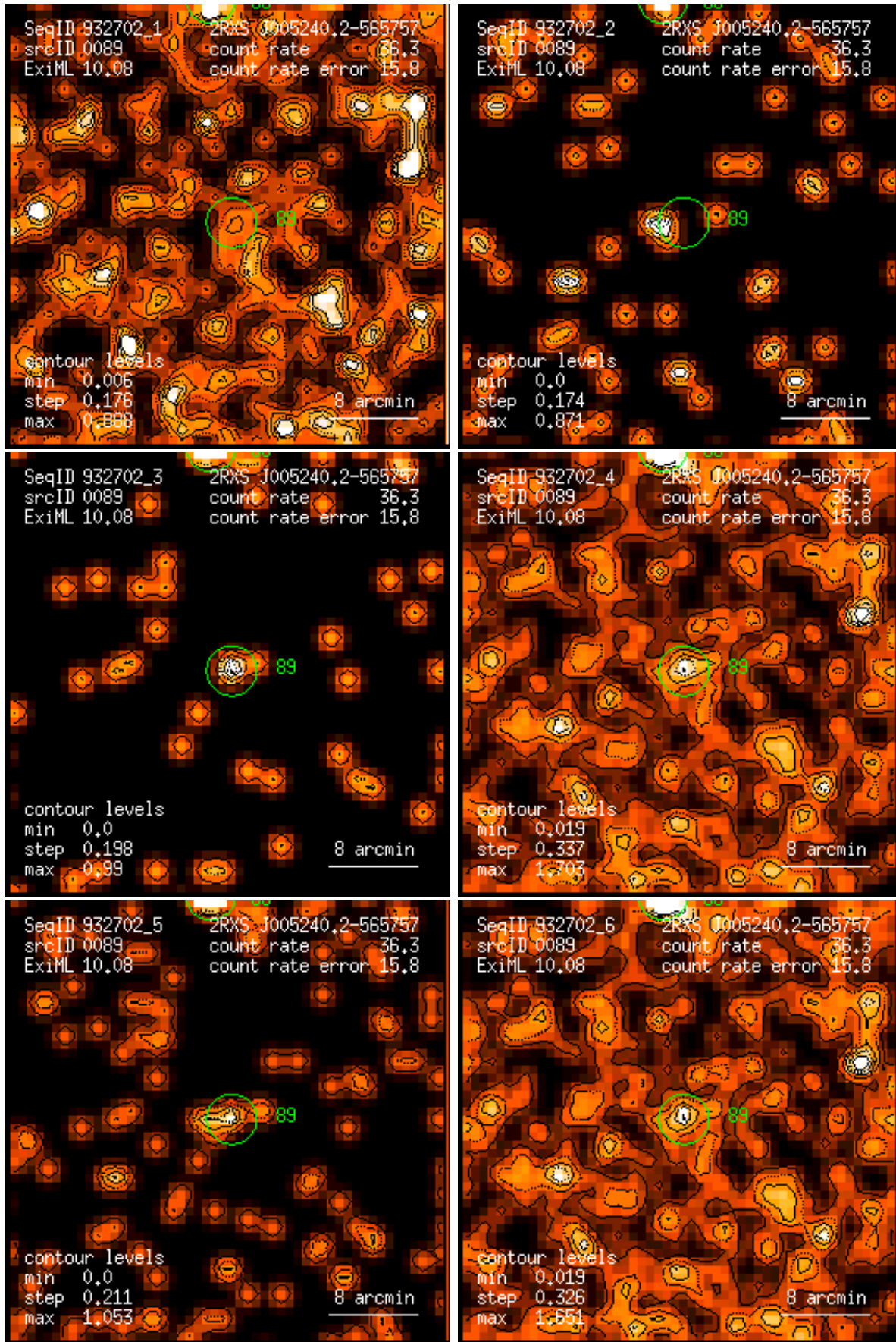
Figure 89: RASS 932702: detection 0089: band rate images, Gaussian filter: (1) PSPC channels 11 – 41, (2) 52 – 90, (3) 91 – 201, (4) 11 – 235, (5) 52 – 201, (6) 11 – 201. Broad band rates in counts/ks. Band rate contour levels in counts/ks/arcmin 2 .
