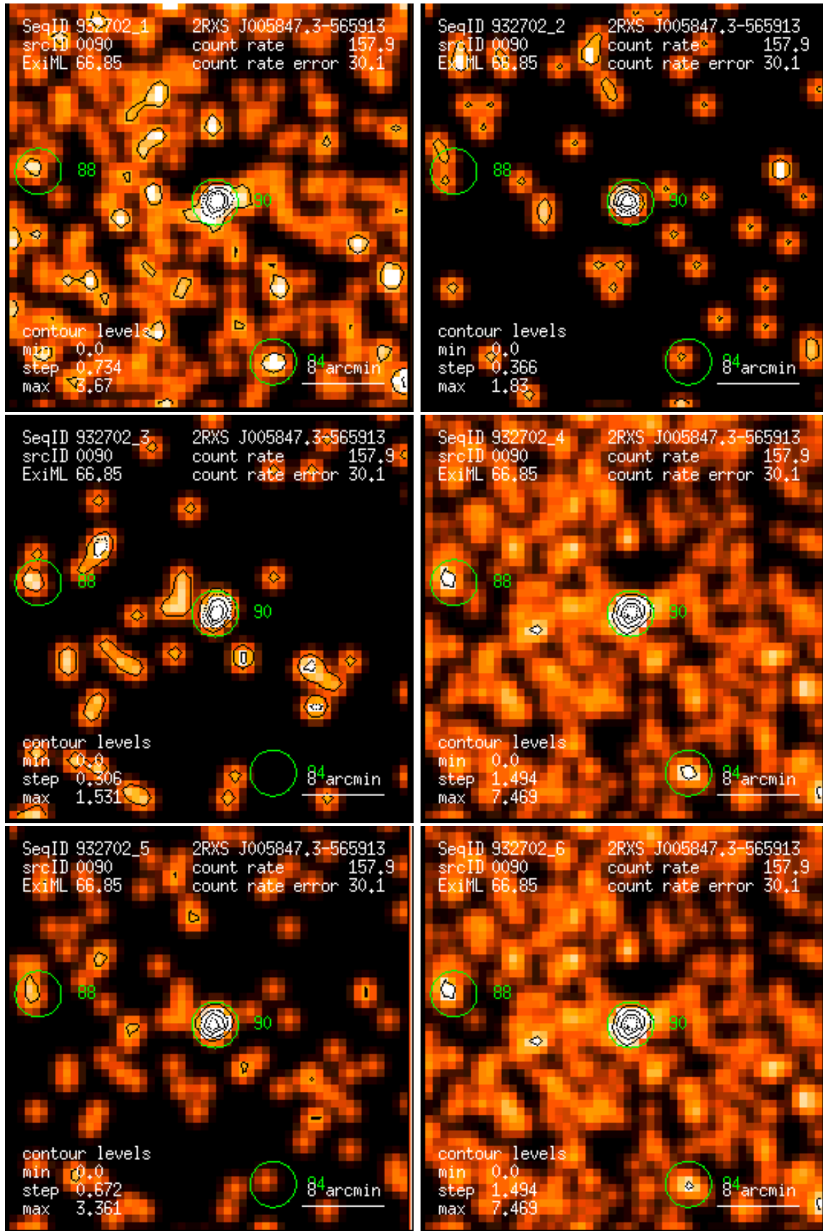
Figure 90: RASS 932702: detection 0090: band rate images, Gaussian filter: (1) PSPC channels 11 – 41, (2) 52 – 90, (3) 91 – 201, (4) 11 – 235, (5) 52 – 201, (6) 11 – 201. Broad band rates in counts/ks. Band rate contour levels in counts/ks/arcmin 2 .
