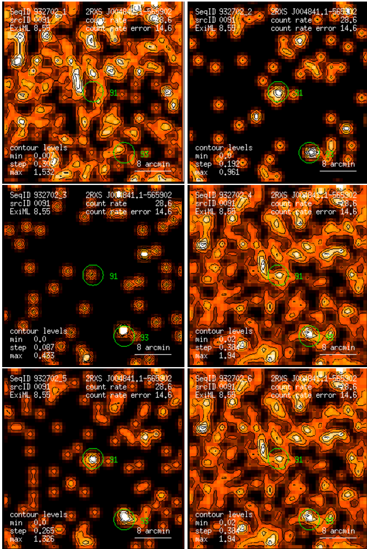
Figure 91: RASS 932702: detection 0091: band rate images, Gaussian filter: (1) PSPC channels 11 – 41, (2) 52 – 90, (3) 91 – 201, (4) 11 – 235, (5) 52 – 201, (6) 11 – 201. Broad band rates in counts/ks. Band rate contour levels in counts/ks/arcmin 2 .
