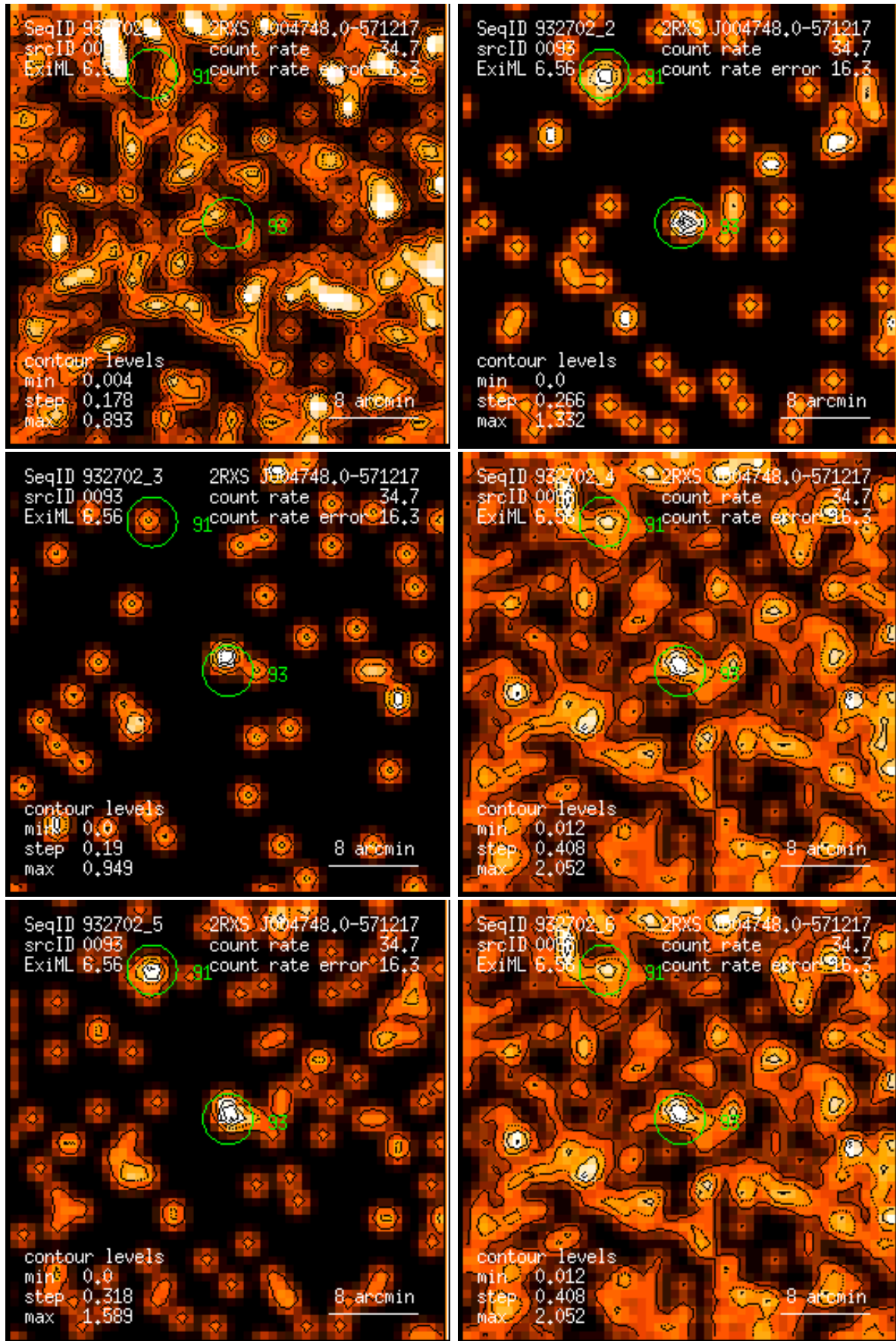
Figure 93: RASS 932702: detection 0093: band rate images, Gaussian filter: (1) PSPC channels 11 – 41, (2) 52 – 90, (3) 91 – 201, (4) 11 – 235, (5) 52 – 201, (6) 11 – 201. Broad band rates in counts/ks. Band rate contour levels in counts/ks/arcmin 2 .
