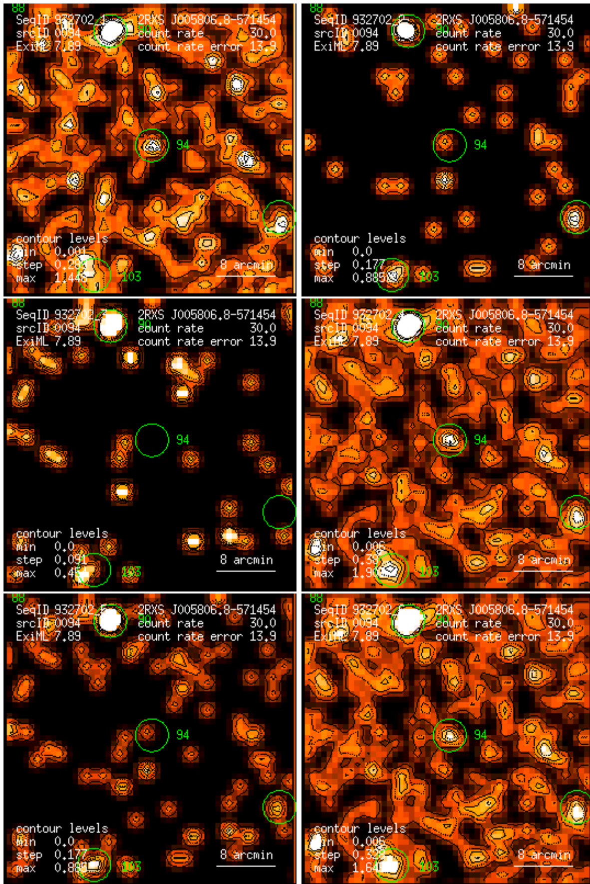
Figure 94: RASS 932702: detection 0094: band rate images, Gaussian filter: (1) PSPC channels 11 – 41, (2) 52 – 90, (3) 91 – 201, (4) 11 – 235, (5) 52 – 201, (6) 11 – 201. Broad band rates in counts/ks. Band rate contour levels in counts/ks/arcmin 2 .
