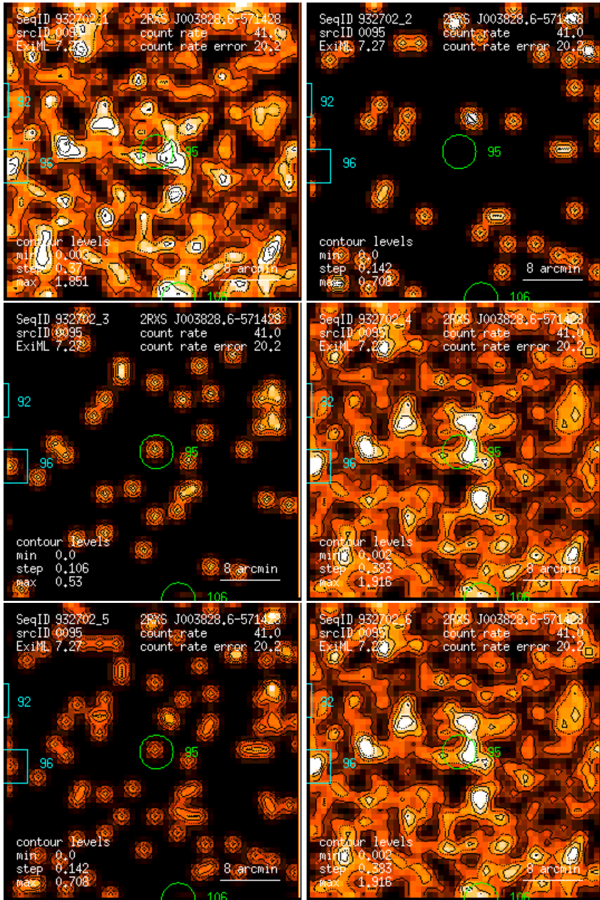
Figure 95: RASS 932702: detection 0095: band rate images, Gaussian filter: (1) PSPC channels 11 – 41, (2) 52 – 90, (3) 91 – 201, (4) 11 – 235, (5) 52 – 201, (6) 11 – 201. Broad band rates in counts/ks. Band rate contour levels in counts/ks/arcmin 2 .
