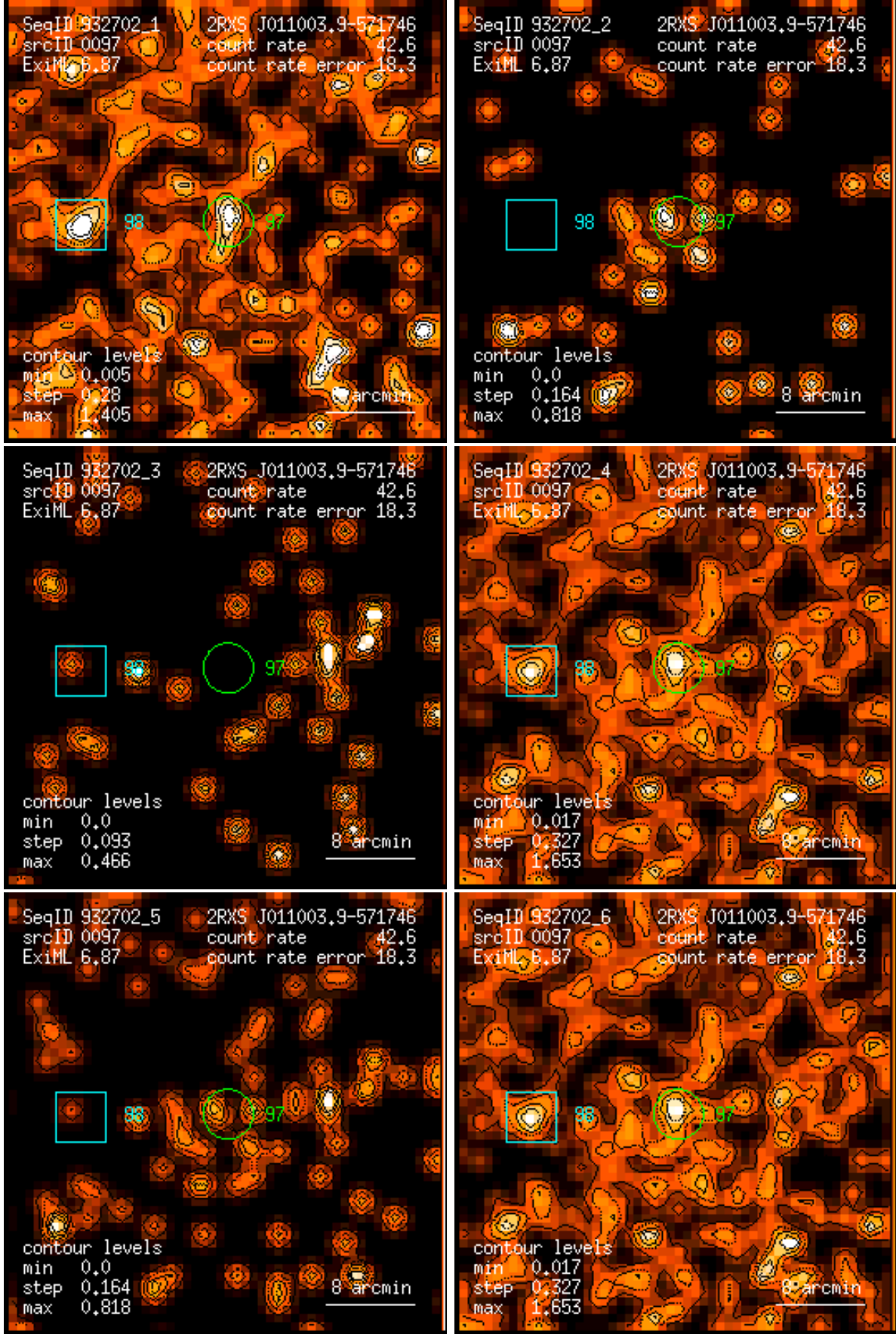
Figure 97: RASS 932702: detection 0097: band rate images, Gaussian filter: (1) PSPC channels 11 – 41, (2) 52 – 90, (3) 91 – 201, (4) 11 – 235, (5) 52 – 201, (6) 11 – 201. Broad band rates in counts/ks. Band rate contour levels in counts/ks/arcmin 2 .
