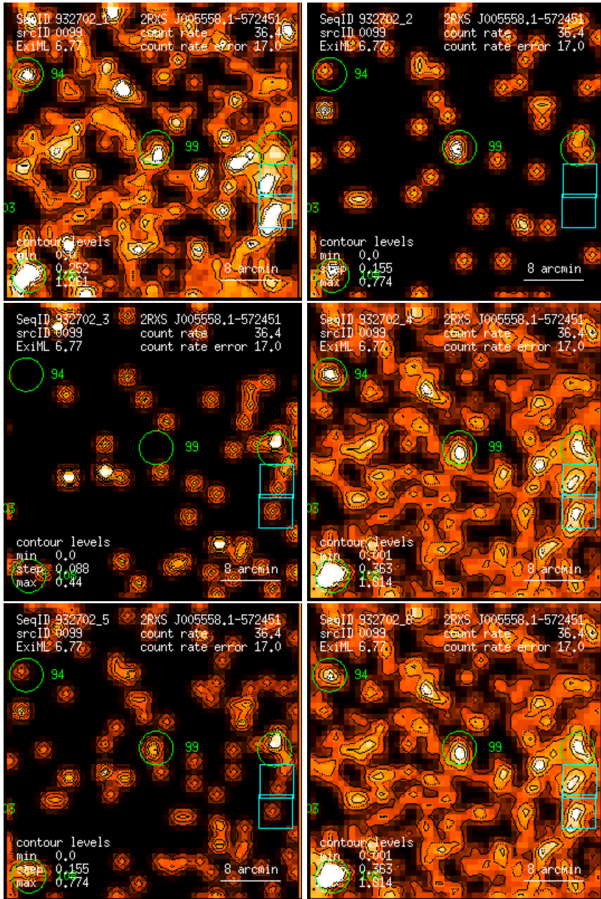
Figure 99: RASS 932702: detection 0099: band rate images, Gaussian filter: (1) PSPC channels 11 – 41, (2) 52 – 90, (3) 91 – 201, (4) 11 – 235, (5) 52 – 201, (6) 11 – 201. Broad band rates in counts/ks. Band rate contour levels in counts/ks/arcmin 2 .
