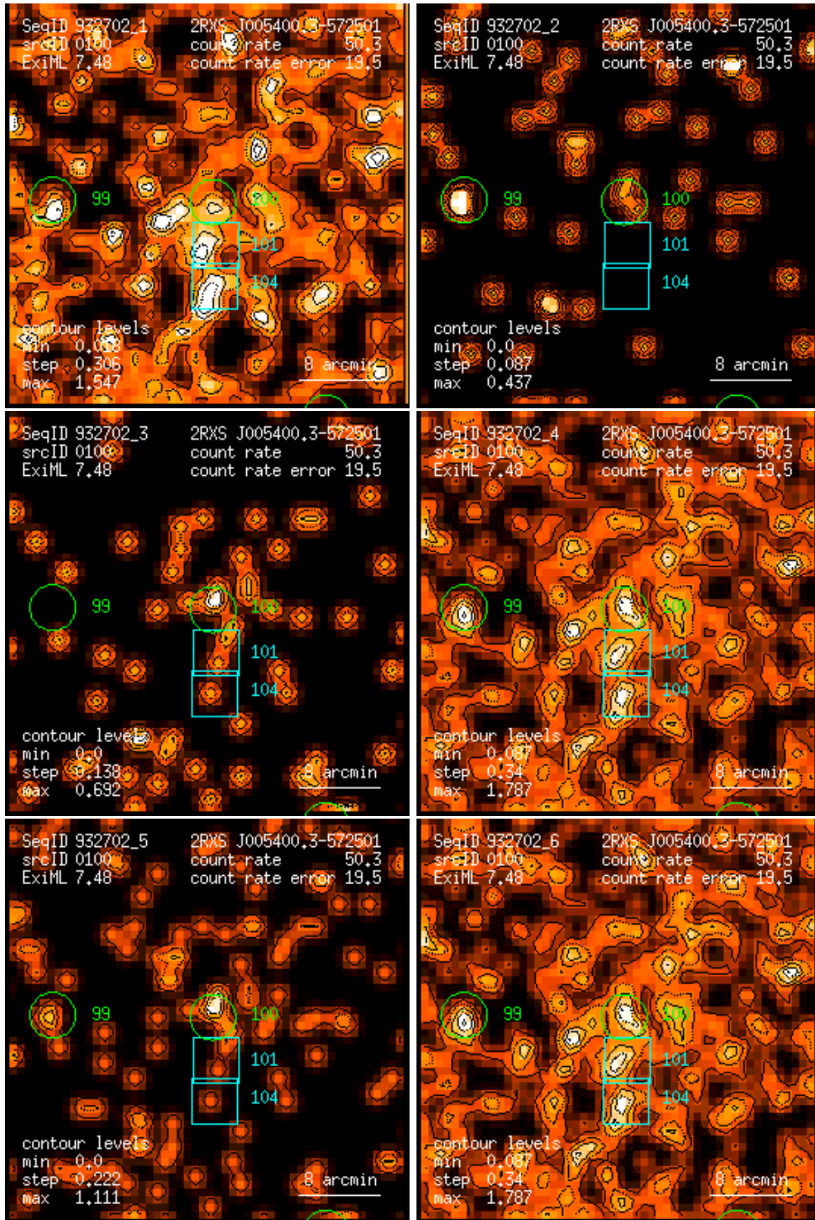
Figure 100: RASS 932702: detection 0100: band rate images, Gaussian filter: (1) PSPC channels 11 – 41, (2) 52 – 90, (3) 91 – 201, (4) 11 – 235, (5) 52 – 201, (6) 11 – 201. Broad band rates in counts/ks. Band rate contour levels in counts/ks/arcmin 2 .
