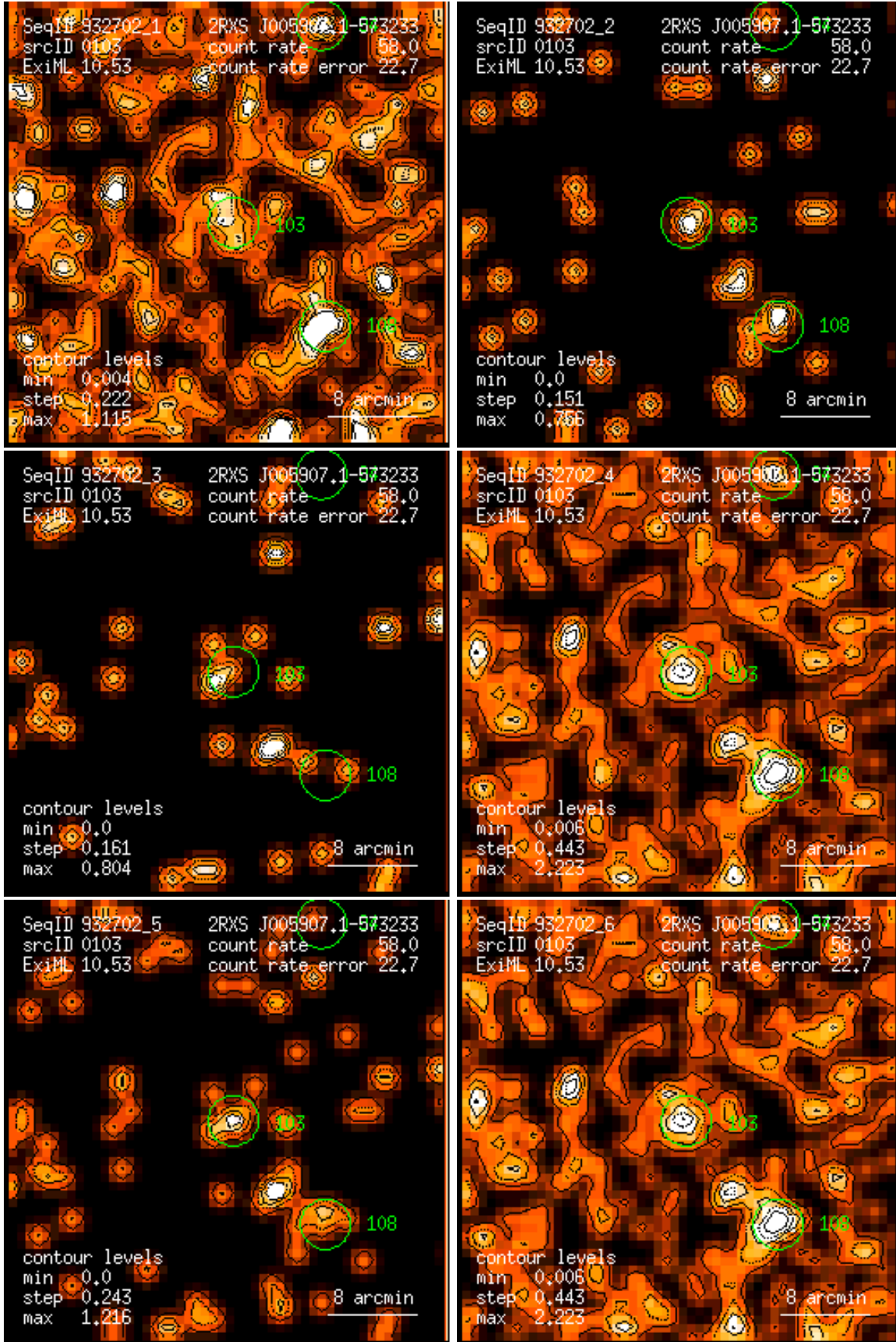
Figure 103: RASS 932702: detection 0103: band rate images, Gaussian filter: (1) PSPC channels 11 – 41, (2) 52 – 90, (3) 91 – 201, (4) 11 – 235, (5) 52 – 201, (6) 11 – 201. Broad band rates in counts/ks. Band rate contour levels in counts/ks/arcmin 2 .
