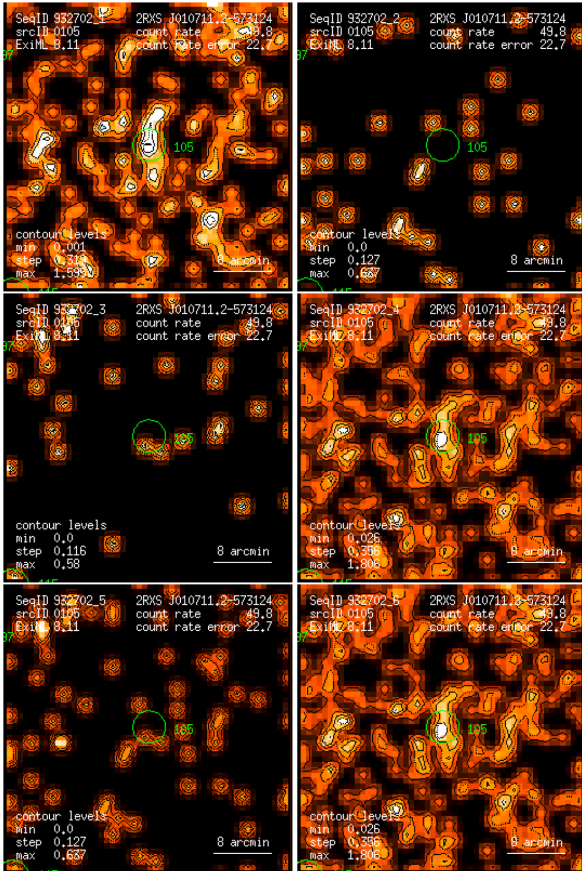
Figure 105: RASS 932702: detection 0105: band rate images, Gaussian filter: (1) PSPC channels 11 – 41, (2) 52 – 90, (3) 91 – 201, (4) 11 – 235, (5) 52 – 201, (6) 11 – 201. Broad band rates in counts/ks. Band rate contour levels in counts/ks/arcmin 2 .
