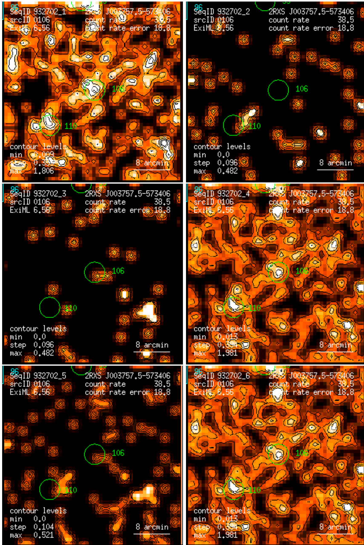
Figure 106: RASS 932702: detection 0106: band rate images, Gaussian filter: (1) PSPC channels 11 – 41, (2) 52 – 90, (3) 91 – 201, (4) 11 – 235, (5) 52 – 201, (6) 11 – 201. Broad band rates in counts/ks. Band rate contour levels in counts/ks/arcmin 2 .
