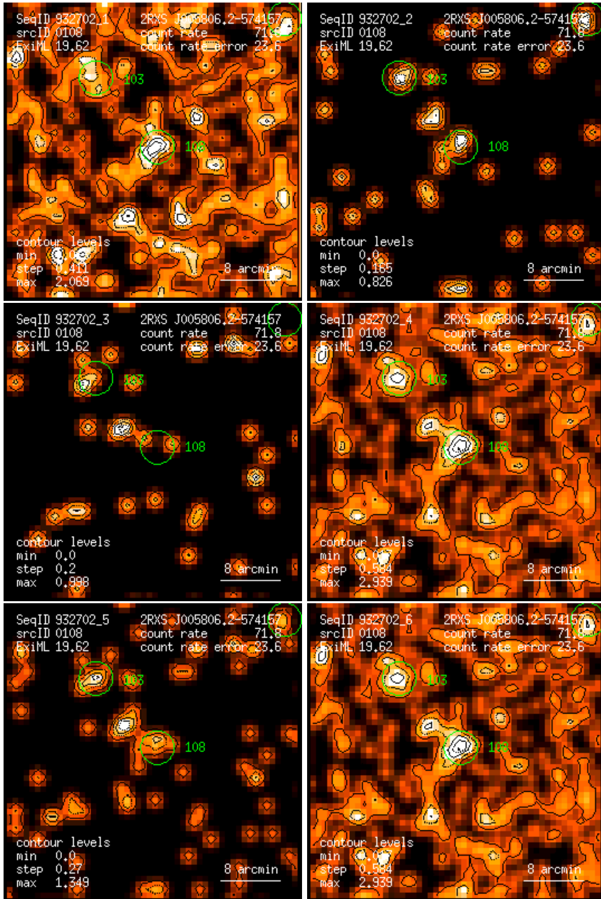
Figure 108: RASS 932702: detection 0108: band rate images, Gaussian filter: (1) PSPC channels 11 – 41, (2) 52 – 90, (3) 91 – 201, (4) 11 – 235, (5) 52 – 201, (6) 11 – 201. Broad band rates in counts/ks. Band rate contour levels in counts/ks/arcmin 2 .
