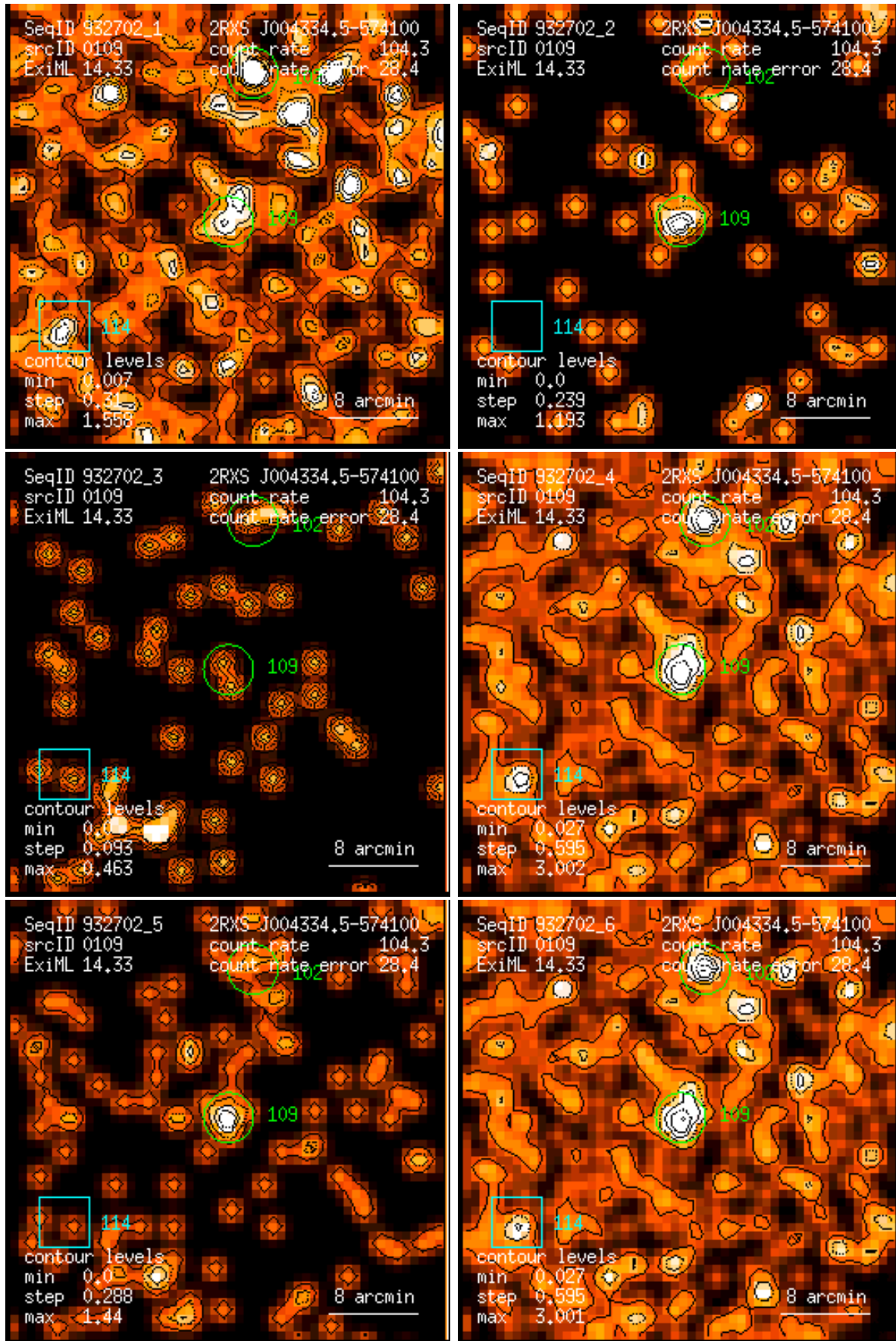
Figure 109: RASS 932702: detection 0109: band rate images, Gaussian filter: (1) PSPC channels 11 – 41, (2) 52 – 90, (3) 91 – 201, (4) 11 – 235, (5) 52 – 201, (6) 11 – 201. Broad band rates in counts/ks. Band rate contour levels in counts/ks/arcmin 2 .
