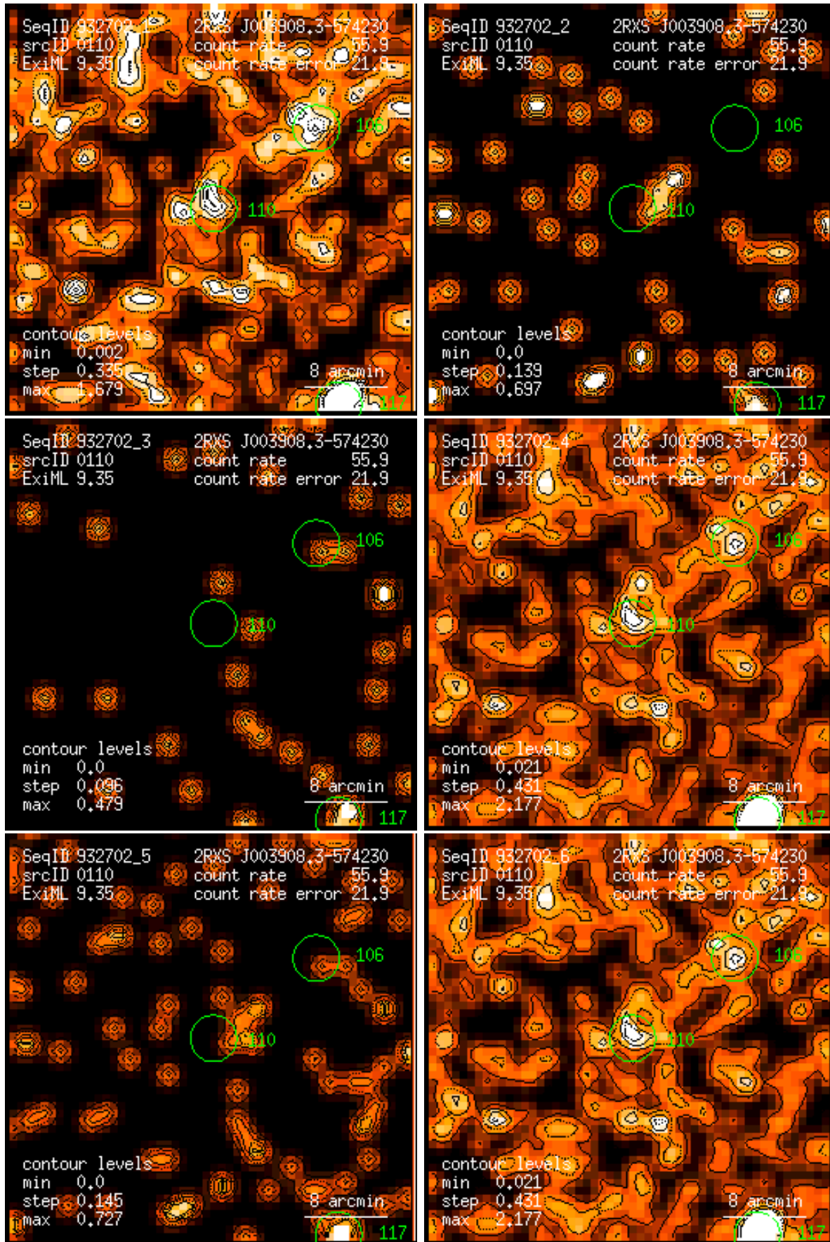
Figure 110: RASS 932702: detection 0110: band rate images, Gaussian filter: (1) PSPPC channels 11 – 41, (2) 52 – 90, (3) 91 – 201, (4) 11 – 235, (5) 52 – 201, (6) 11 – 201. Broad band rates in counts/ks. Band rate contour levels in counts/ks/arcmin 2 .
