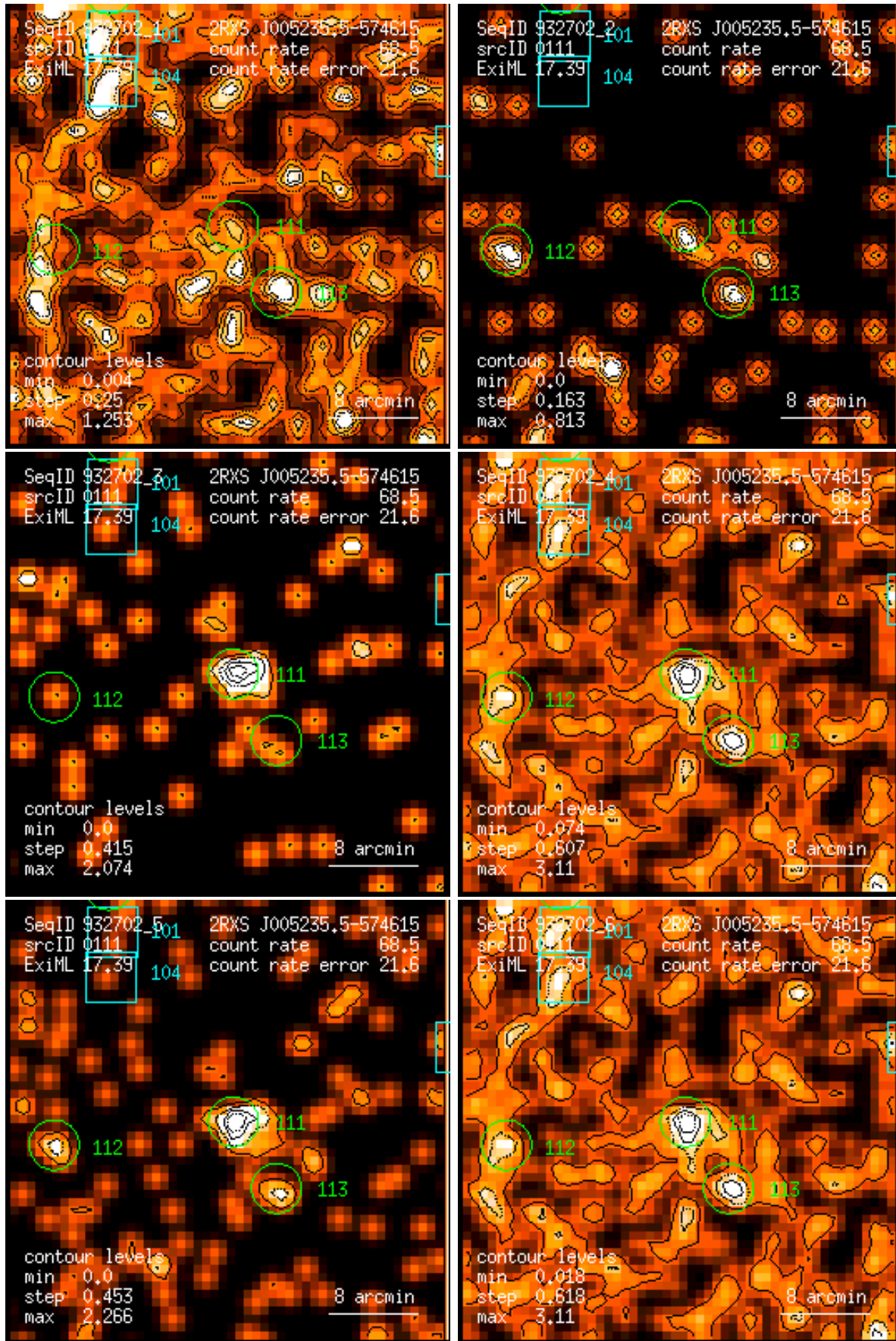
Figure 111: RASS 932702: detection 0111: band rate images, Gaussian filter: (1) PSPC channels 11 – 41, (2) 52 – 90, (3) 91 – 201, (4) 11 – 235, (5) 52 – 201, (6) 11 – 201. Broad band rates in counts/ks. Band rate contour levels in counts/ks/arcmin 2 .
