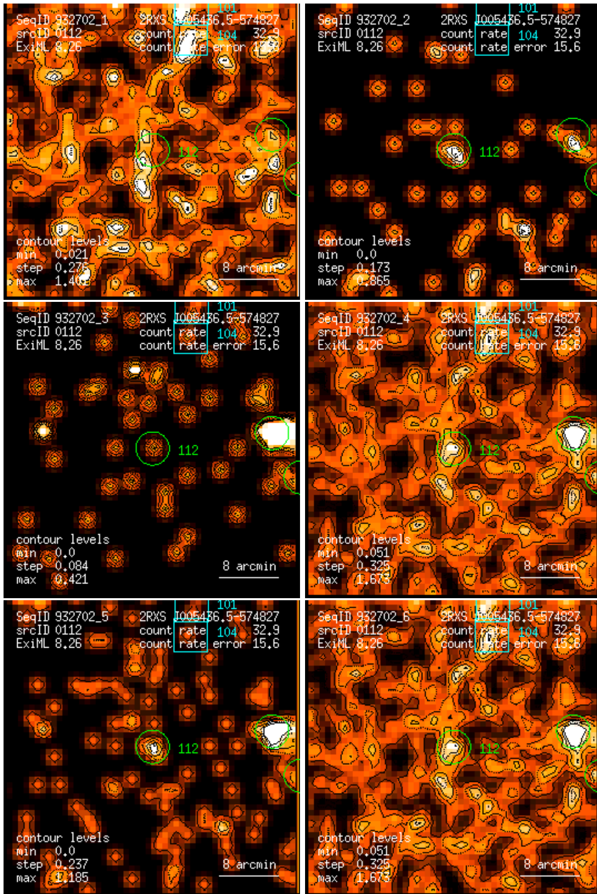
Figure 112: RASS 932702: detection 0112: band rate images, Gaussian filter: (1) PSPC channels 11 – 41, (2) 52 – 90, (3) 91 – 201, (4) 11 – 235, (5) 52 – 201, (6) 11 – 201. Broad band rates in counts/ks. Band rate contour levels in counts/ks/arcmin 2 .
