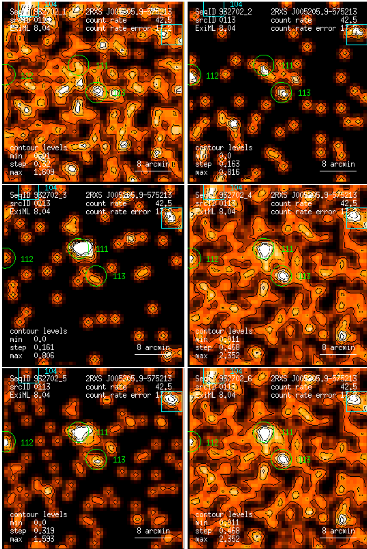
Figure 113: RASS 932702: detection 0113: band rate images, Gaussian filter: (1) PSPC channels 11 – 41, (2) 52 – 90, (3) 91 – 201, (4) 11 – 235, (5) 52 – 201, (6) 11 – 201. Broad band rates in counts/ks. Band rate contour levels in counts/ks/arcmin 2 .
