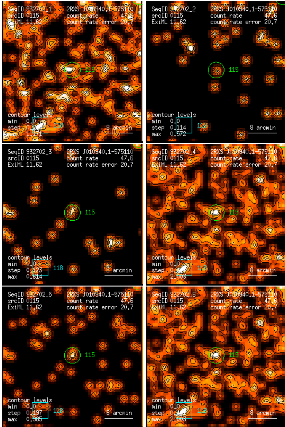
Figure 115: RASS 932702: detection 0115: band rate images, Gaussian filter: (1) PSPC channels 11 – 41, (2) 52 – 90, (3) 91 – 201, (4) 11 – 235, (5) 52 – 201, (6) 11 – 201. Broad band rates in counts/ks. Band rate contour levels in counts/ks/arcmin 2 .
