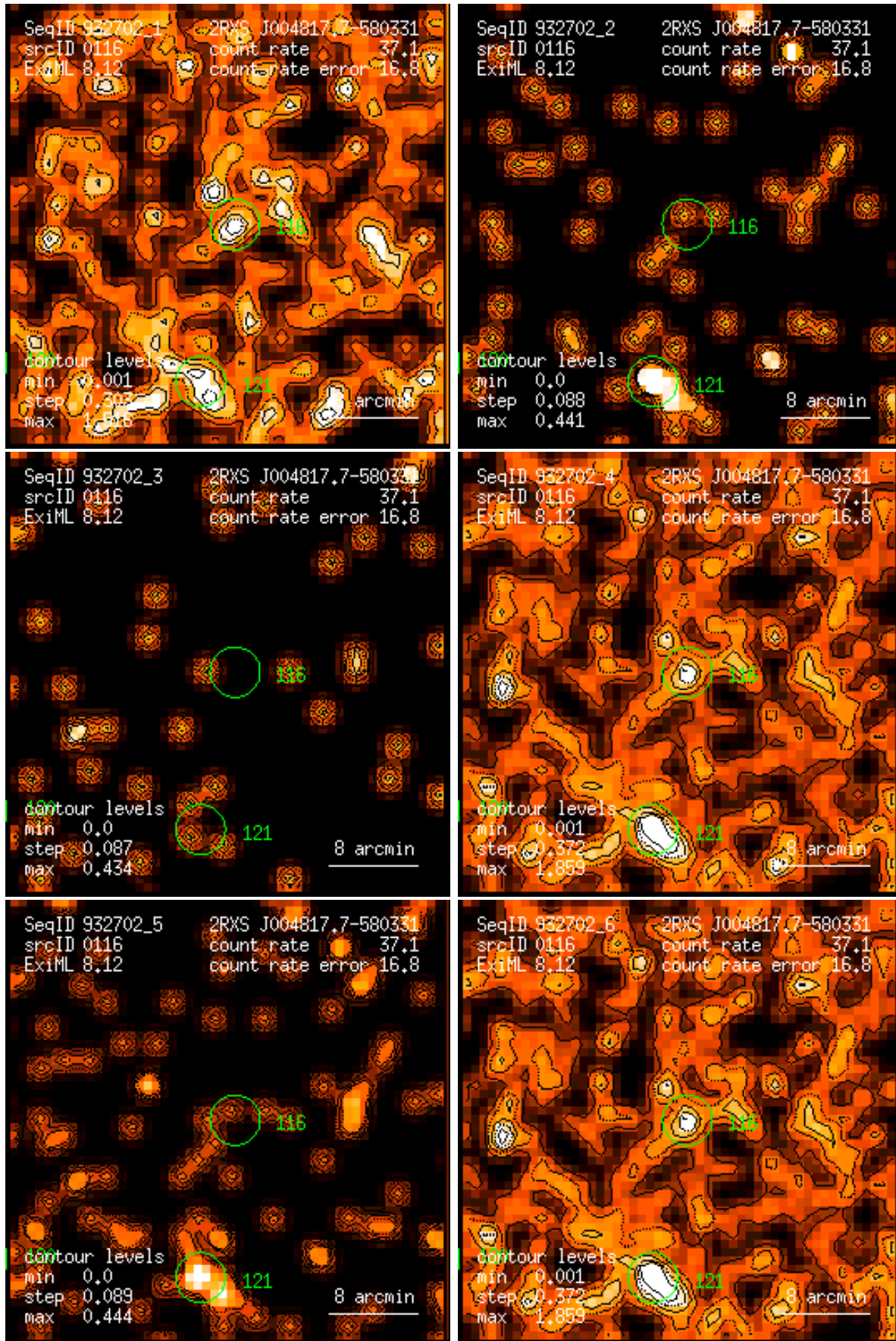
Figure 116: RASS 932702: detection 0116: band rate images, Gaussian filter: (1) PSPC channels 11 – 41, (2) 52 – 90, (3) 91 – 201, (4) 11 – 235, (5) 52 – 201, (6) 11 – 201. Broad band rates in counts/ks. Band rate contour levels in counts/ks/arcmin 2 .
