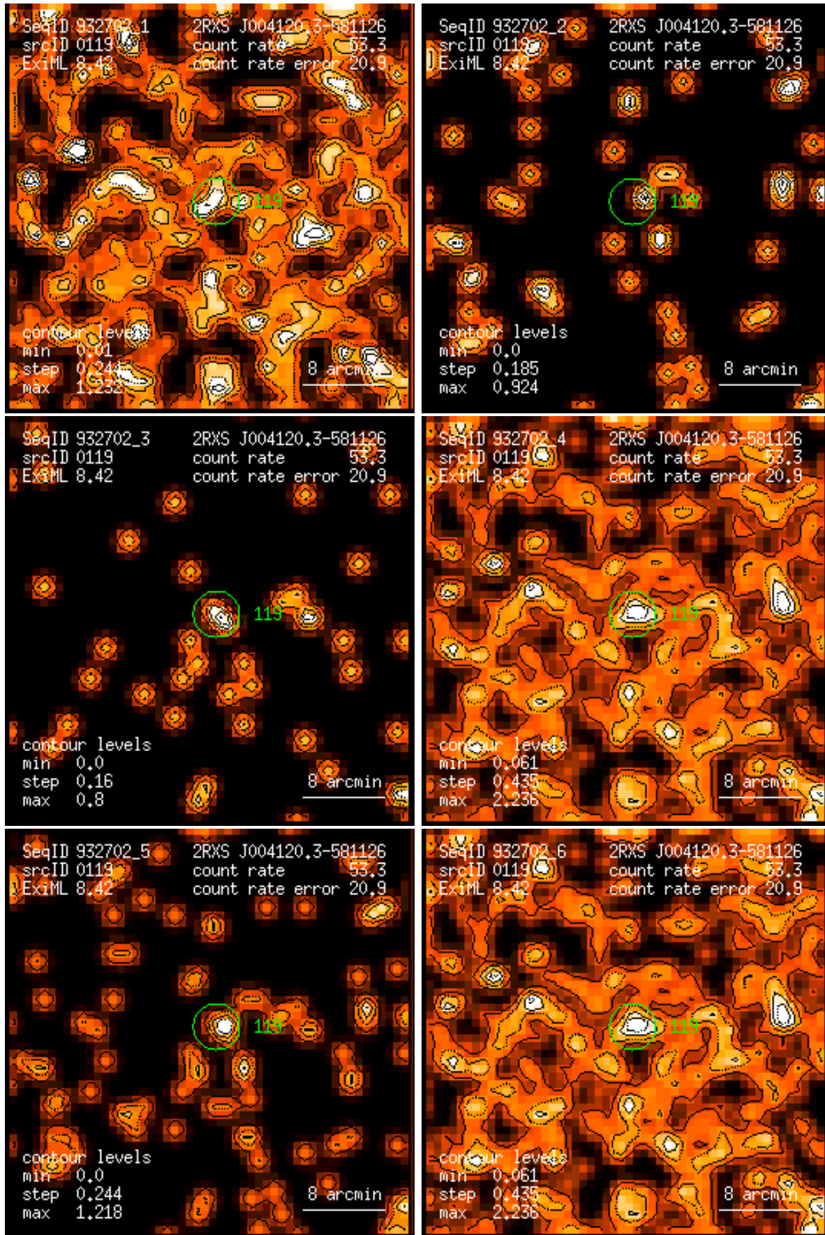
Figure 119: RASS 932702: detection 0119: band rate images, Gaussian filter: (1) PSPC channels 11 – 41, (2) 52 – 90, (3) 91 – 201, (4) 11 – 235, (5) 52 – 201, (6) 11 – 201. Broad band rates in counts/ks. Band rate contour levels in counts/ks/arcmin 2 .
