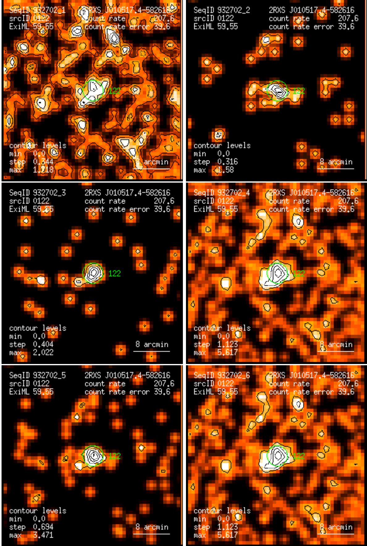
Figure 122: RASS 932702: detection 0122: band rate images, Gaussian filter: (1) PSPC channels 11 – 41, (2) 52 – 90, (3) 91 – 201, (4) 11 – 235, (5) 52 – 201, (6) 11 – 201. Broad band rates in counts/ks. Band rate contour levels in counts/ks/arcmin 2 .
