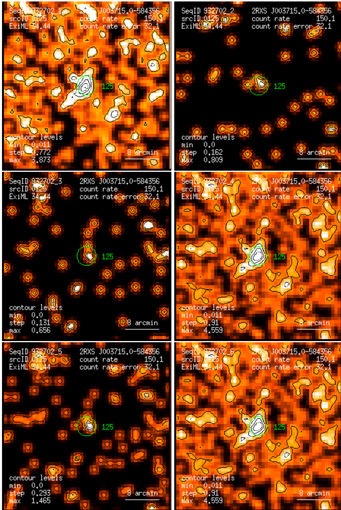
Figure 125: RASS 932702: detection 0125: band rate images, Gaussian filter: (1) PSPC channels 11 – 41, (2) 52 – 90, (3) 91 – 201, (4) 11 – 235, (5) 52 – 201, (6) 11 – 201. Broad band rates in counts/ks. Band rate contour levels in counts/ks/arcmin 2 .
