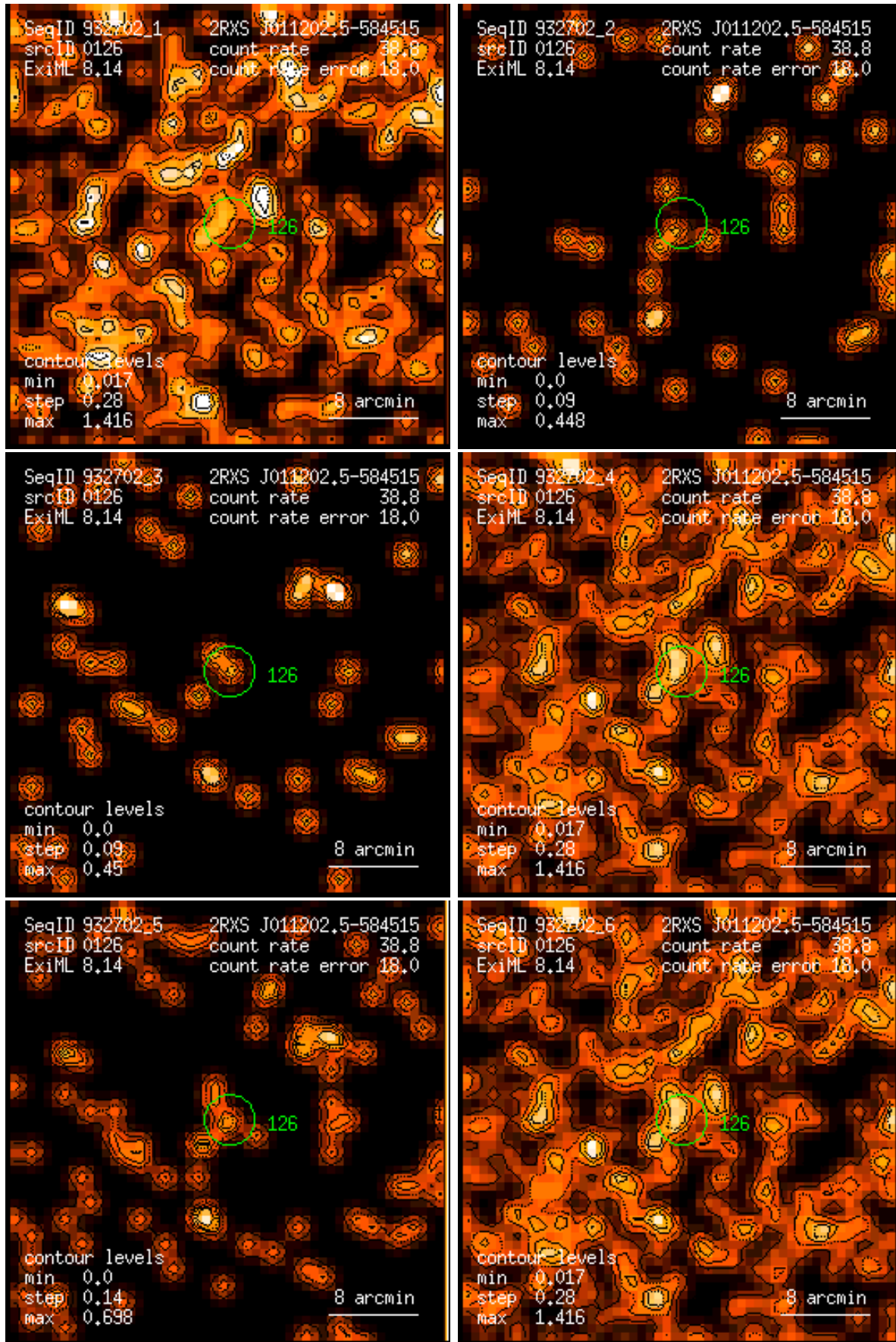
Figure 126: RASS 932702: detection 0126: band rate images, Gaussian filter: (1) PSPC channels 11 – 41, (2) 52 – 90, (3) 91 – 201, (4) 11 – 235, (5) 52 – 201, (6) 11 – 201. Broad band rates in counts/ks. Band rate contour levels in counts/ks/arcmin 2 .
