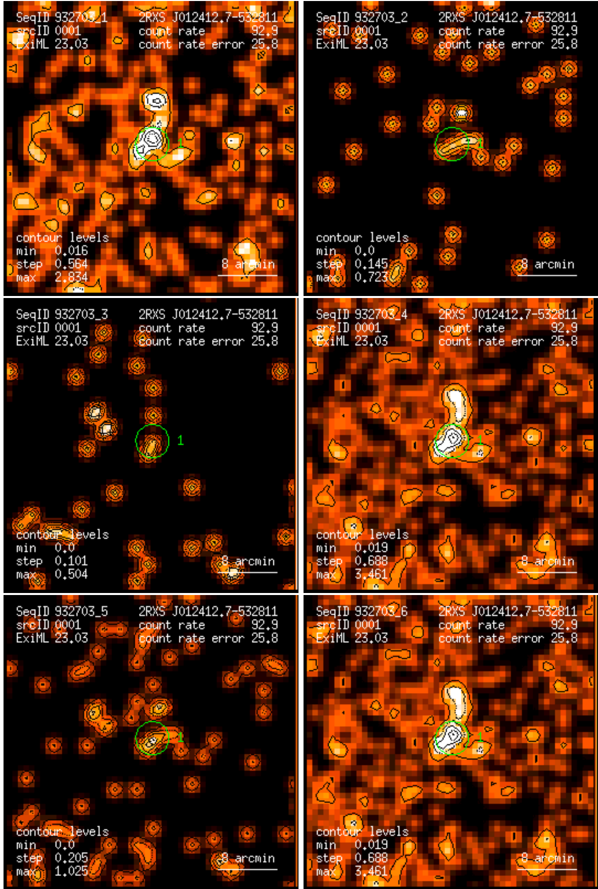
Figure 1: RASS 932703: detection 0001: band rate images, Gaussian filter: (1) PSPC channels 11 – 41, (2) 52 – 90, (3) 91 – 201, (4) 11 – 235, (5) 52 – 201, (6) 11 – 201. Broad band rates in counts/ks. Band rate contour levels in counts/ks/arcmin 2 .
