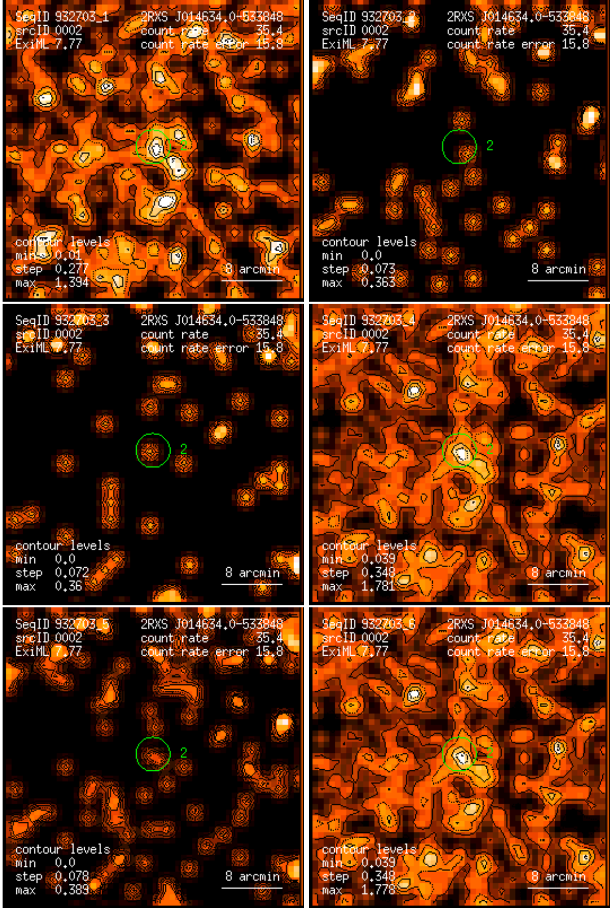
Figure 2: RASS 932703: detection 0002: band rate images, Gaussian filter: (1) PSPC channels 11 – 41, (2) 52 – 90, (3) 91 – 201, (4) 11 – 235, (5) 52 – 201, (6) 11 – 201. Broad band rates in counts/ks. Band rate contour levels in counts/ks/arcmin 2 .
