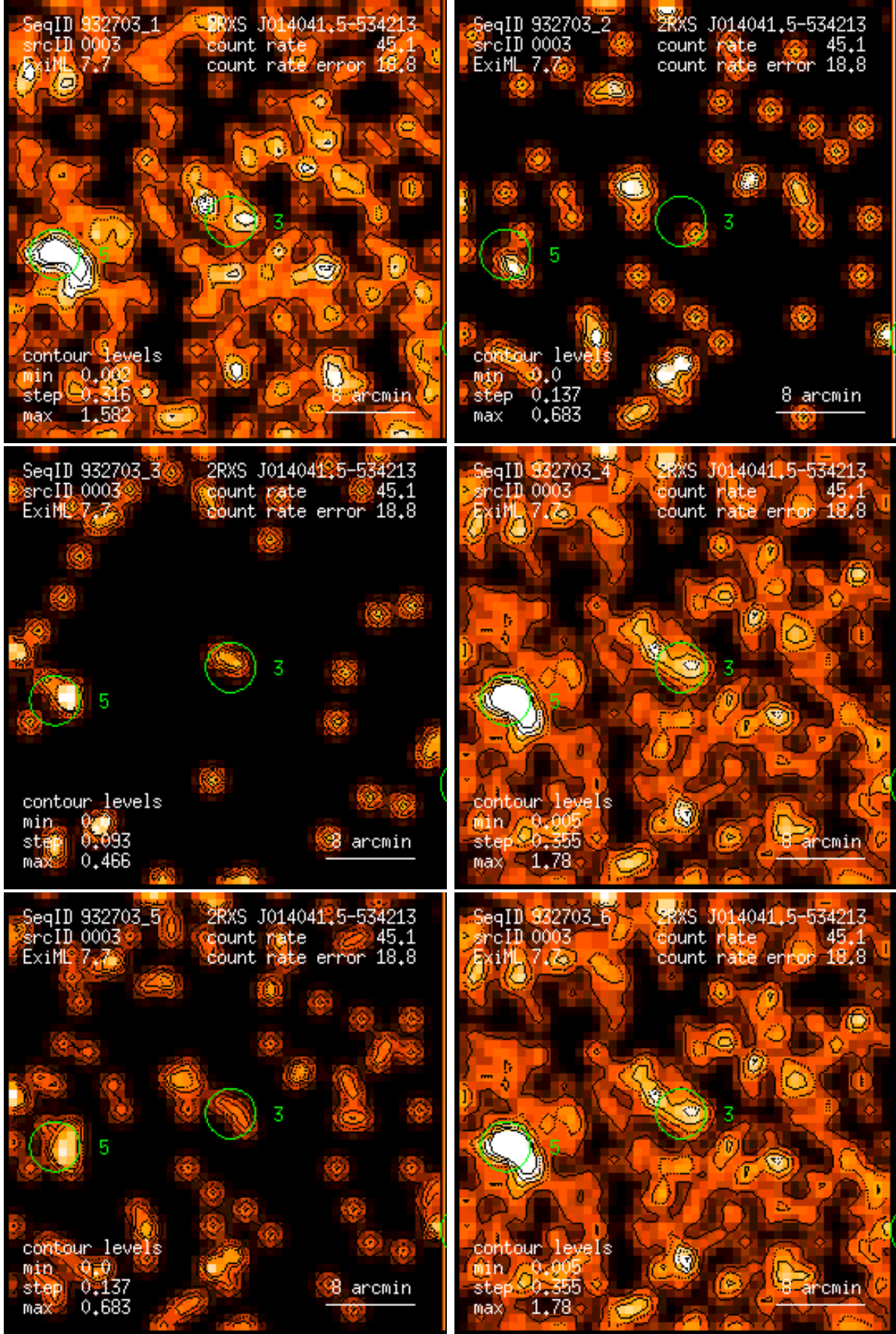
Figure 3: RASS 932703: detection 0003: band rate images, Gaussian filter: (1) PSPC channels 11 – 41, (2) 52 – 90, (3) 91 – 201, (4) 11 – 235, (5) 52 – 201, (6) 11 – 201. Broad band rates in counts/ks. Band rate contour levels in counts/ks/arcmin 2 .
