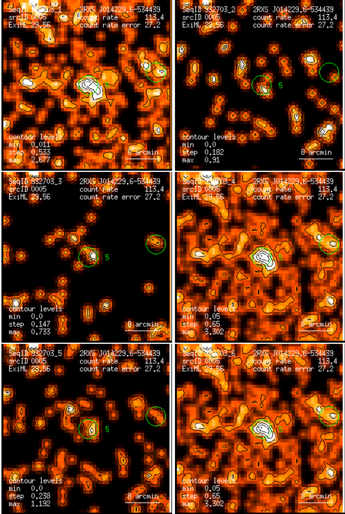
Figure 5: RASS 932703: detection 0005: band rate images, Gaussian filter: (1) PSPC channels 11 – 41, (2) 52 – 90, (3) 91 – 201, (4) 11 – 235, (5) 52 – 201, (6) 11 – 201. Broad band rates in counts/ks. Band rate contour levels in counts/ks/arcmin 2 .
