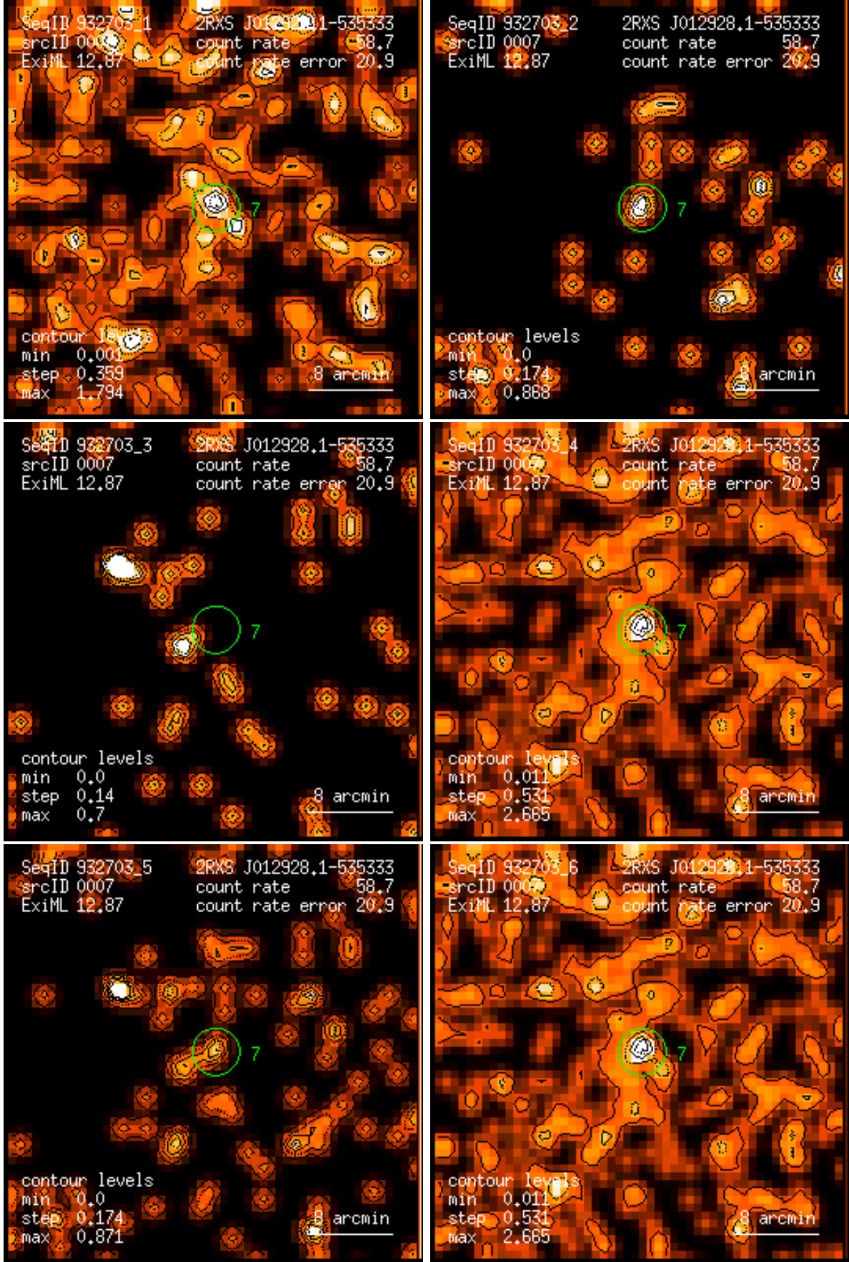
Figure 7: RASS 932703: detection 0007: band rate images, Gaussian filter: (1) PSPC channels 11 – 41, (2) 52 – 90, (3) 91 – 201, (4) 11 – 235, (5) 52 – 201, (6) 11 – 201. Broad band rates in counts/ks. Band rate contour levels in counts/ks/arcmin 2 .
