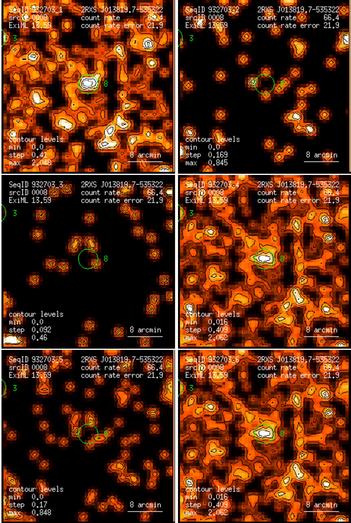
Figure 8: RASS 932703: detection 0008: band rate images, Gaussian filter: (1) PSPC channels 11 – 41, (2) 52 – 90, (3) 91 – 201, (4) 11 – 235, (5) 52 – 201, (6) 11 – 201. Broad band rates in counts/ks. Band rate contour levels in counts/ks/arcmin 2 .
