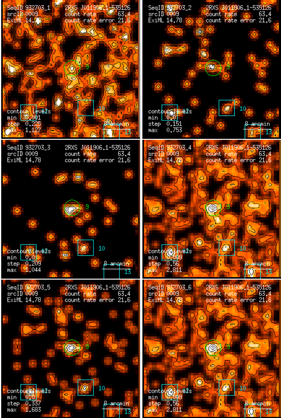
Figure 9: RASS 932703: detection 0009: band rate images, Gaussian filter: (1) PSPC channels 11 – 41, (2) 52 – 90, (3) 91 – 201, (4) 11 – 235, (5) 52 – 201, (6) 11 – 201. Broad band rates in counts/ks. Band rate contour levels in counts/ks/arcmin 2 .
