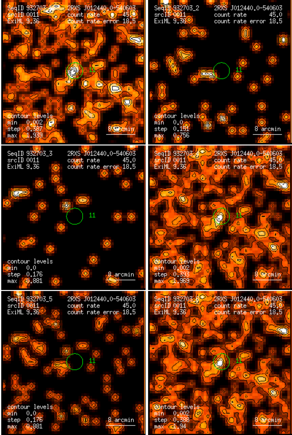
Figure 11: RASS 932703: detection 0011: band rate images, Gaussian filter: (1) PSPC channels 11 – 41, (2) 52 – 90, (3) 91 – 201, (4) 11 – 235, (5) 52 – 201, (6) 11 – 201. Broad band rates in counts/ks. Band rate contour levels in counts/ks/arcmin 2 .
