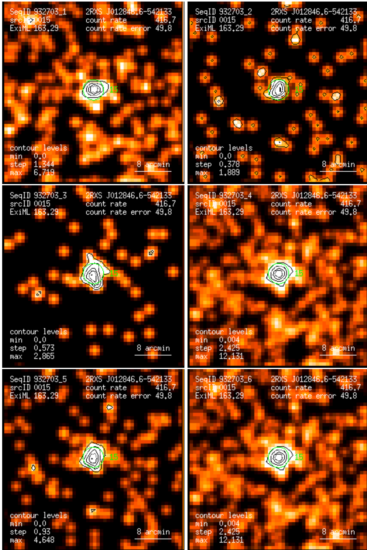
Figure 15: RASS 932703: detection 0015: band rate images, Gaussian filter: (1) PSPC channels 11 – 41, (2) 52 – 90, (3) 91 – 201, (4) 11 – 235, (5) 52 – 201, (6) 11 – 201. Broad band rates in counts/ks. Band rate contour levels in counts/ks/arcmin 2 .
