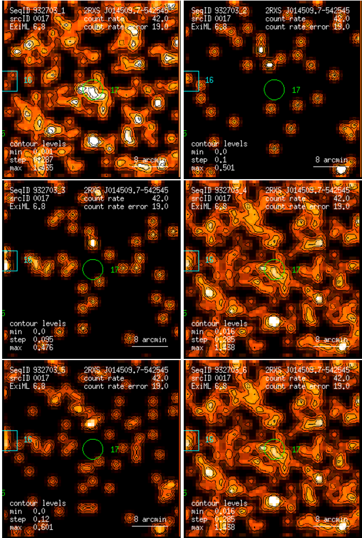
Figure 17: RASS 932703: detection 0017: band rate images, Gaussian filter: (1) PSPC channels 11 – 41, (2) 52 – 90, (3) 91 – 201, (4) 11 – 235, (5) 52 – 201, (6) 11 – 201. Broad band rates in counts/ks. Band rate contour levels in counts/ks/arcmin 2 .
