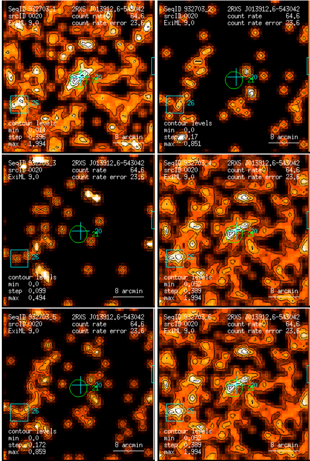
Figure 20: RASS 932703: detection 0020: band rate images, Gaussian filter: (1) PSPC channels 11 – 41, (2) 52 – 90, (3) 91 – 201, (4) 11 – 235, (5) 52 – 201, (6) 11 – 201. Broad band rates in counts/ks. Band rate contour levels in counts/ks/arcmin 2 .
