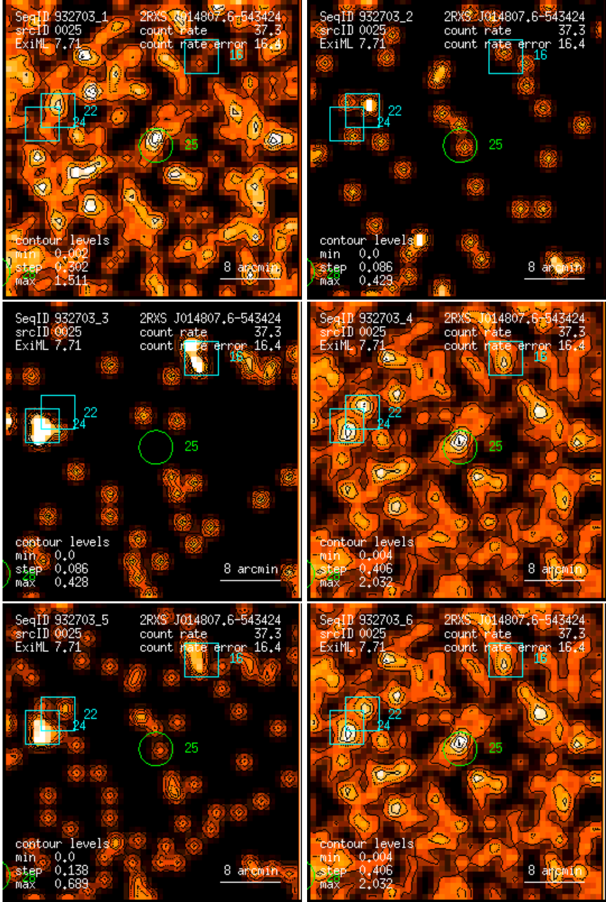
Figure 25: RASS 932703: detection 0025: band rate images, Gaussian filter: (1) PSPC channels 11 – 41, (2) 52 – 90, (3) 91 – 201, (4) 11 – 235, (5) 52 – 201, (6) 11 – 201. Broad band rates in counts/ks. Band rate contour levels in counts/ks/arcmin 2 .
