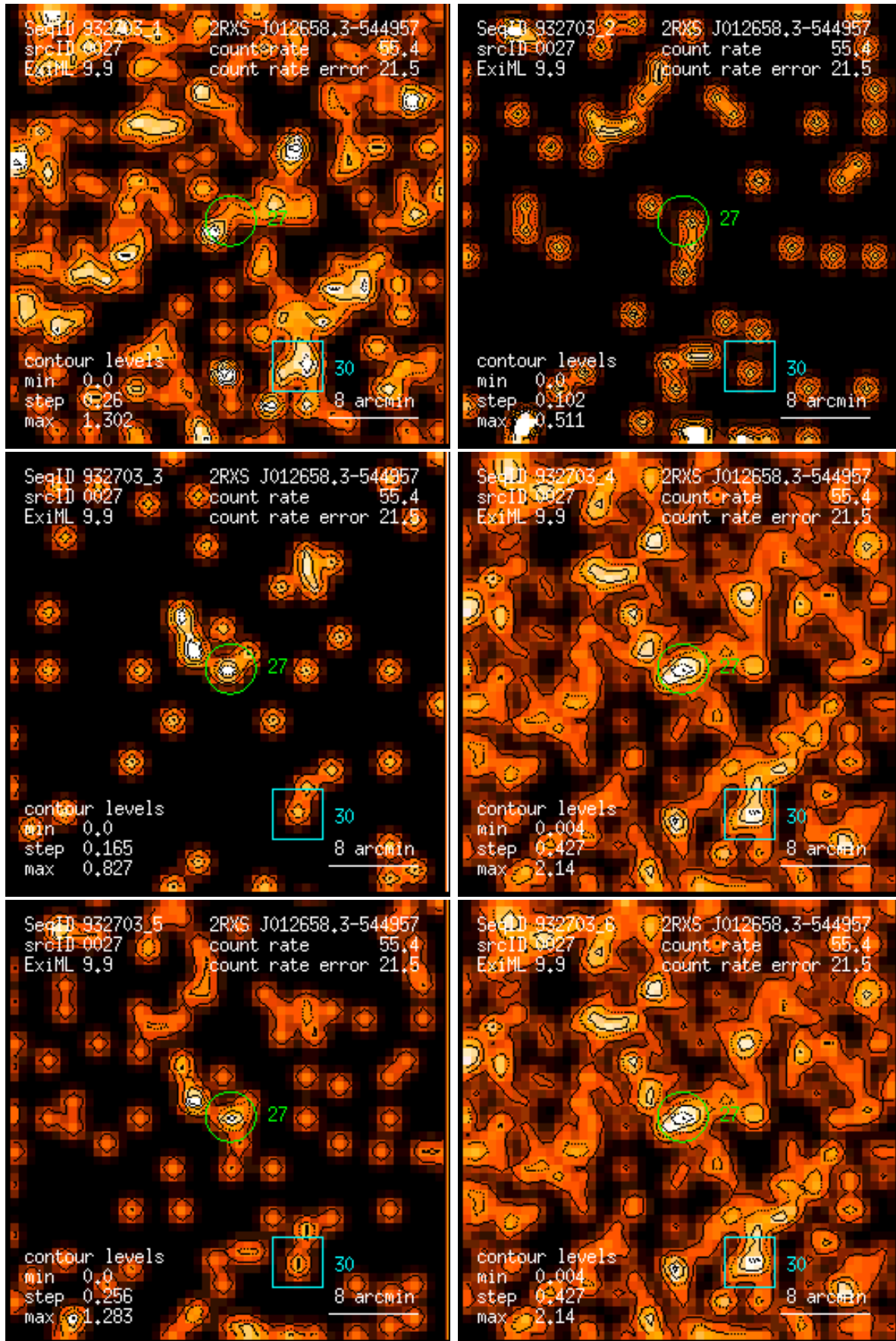
Figure 27: RASS 932703: detection 0027: band rate images, Gaussian filter: (1) PSPC channels 11 – 41, (2) 52 – 90, (3) 91 – 201, (4) 11 – 235, (5) 52 – 201, (6) 11 – 201. Broad band rates in counts/ks. Band rate contour levels in counts/ks/arcmin 2 .
