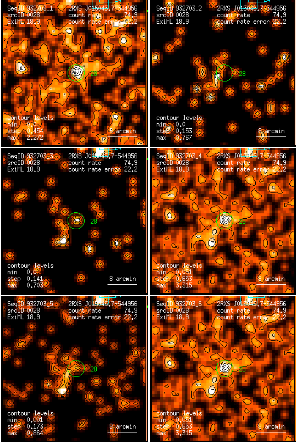
Figure 28: RASS 932703: detection 0028: band rate images, Gaussian filter: (1) PSPC channels 11 – 41, (2) 52 – 90, (3) 91 – 201, (4) 11 – 235, (5) 52 – 201, (6) 11 – 201. Broad band rates in counts/ks. Band rate contour levels in counts/ks/arcmin 2 .
