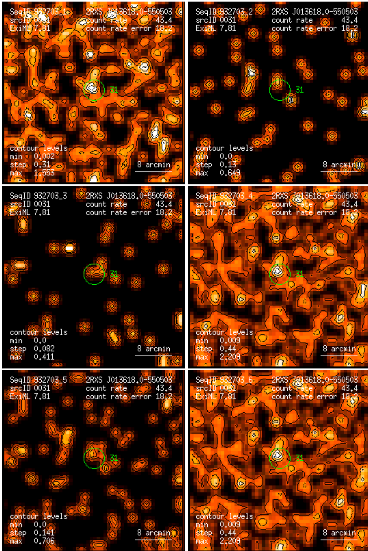
Figure 31: RASS 932703: detection 0031: band rate images, Gaussian filter: (1) PSPC channels 11 – 41, (2) 52 – 90, (3) 91 – 201, (4) 11 – 235, (5) 52 – 201, (6) 11 – 201. Broad band rates in counts/ks. Band rate contour levels in counts/ks/arcmin 2 .
