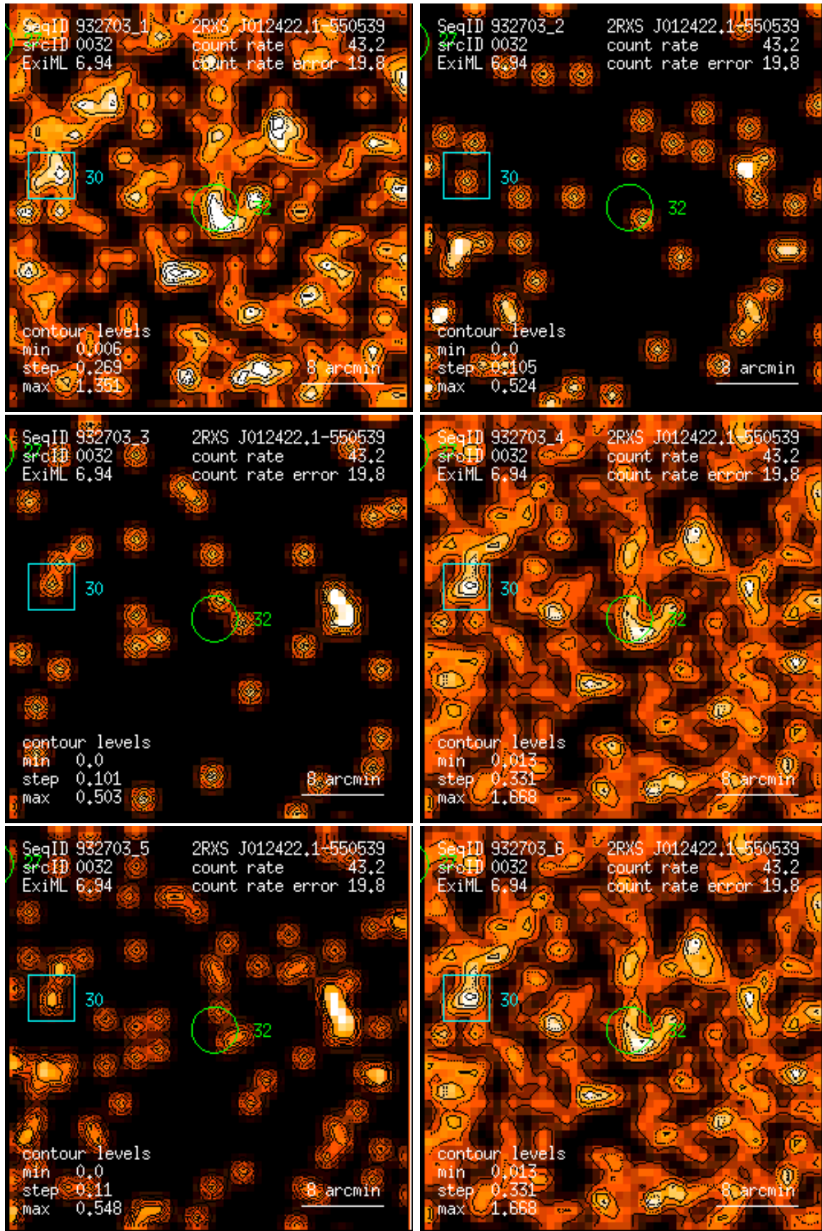
Figure 32: RASS 932703: detection 0032: band rate images, Gaussian filter: (1) PSPC channels 11 – 41, (2) 52 – 90, (3) 91 – 201, (4) 11 – 235, (5) 52 – 201, (6) 11 – 201. Broad band rates in counts/ks. Band rate contour levels in counts/ks/arcmin 2 .
