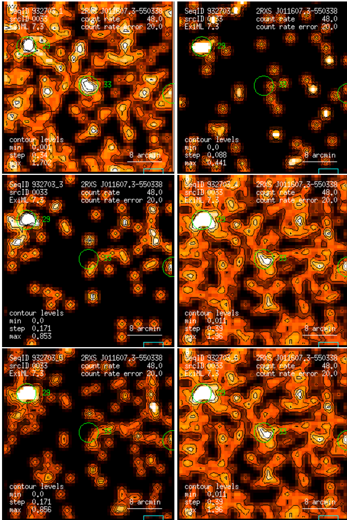
Figure 33: RASS 932703: detection 0033: band rate images, Gaussian filter: (1) PSPC channels 11 – 41, (2) 52 – 90, (3) 91 – 201, (4) 11 – 235, (5) 52 – 201, (6) 11 – 201. Broad band rates in counts/ks. Band rate contour levels in counts/ks/arcmin 2 .
