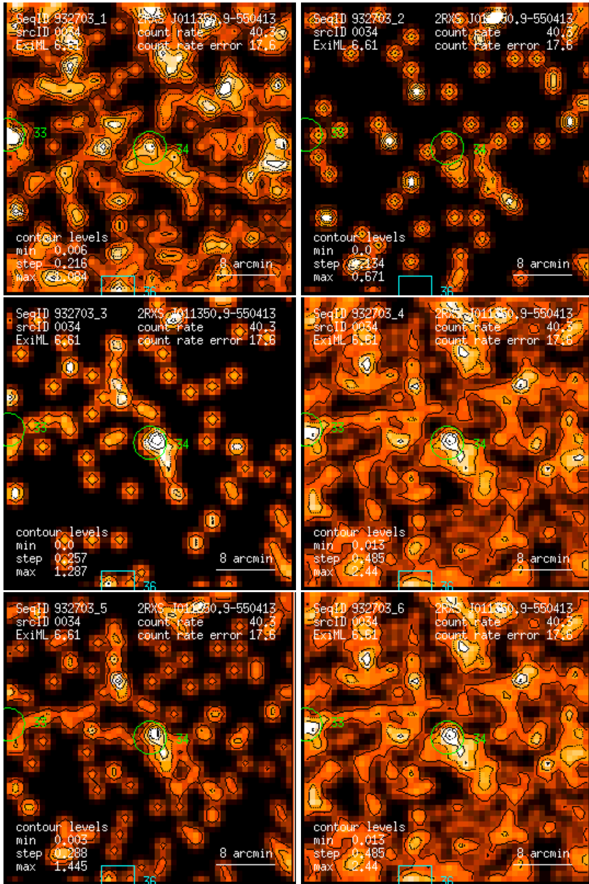
Figure 34: RASS 932703: detection 0034: band rate images, Gaussian filter: (1) PSPC channels 11 – 41, (2) 52 – 90, (3) 91 – 201, (4) 11 – 235, (5) 52 – 201, (6) 11 – 201. Broad band rates in counts/ks. Band rate contour levels in counts/ks/arcmin 2 .
