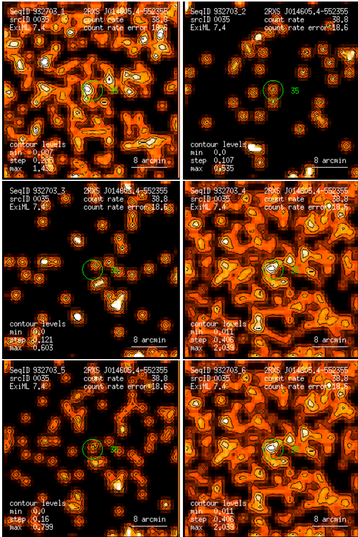
Figure 35: RASS 932703: detection 0035: band rate images, Gaussian filter: (1) PSPC channels 11 – 41, (2) 52 – 90, (3) 91 – 201, (4) 11 – 235, (5) 52 – 201, (6) 11 – 201. Broad band rates in counts/ks. Band rate contour levels in counts/ks/arcmin 2 .
