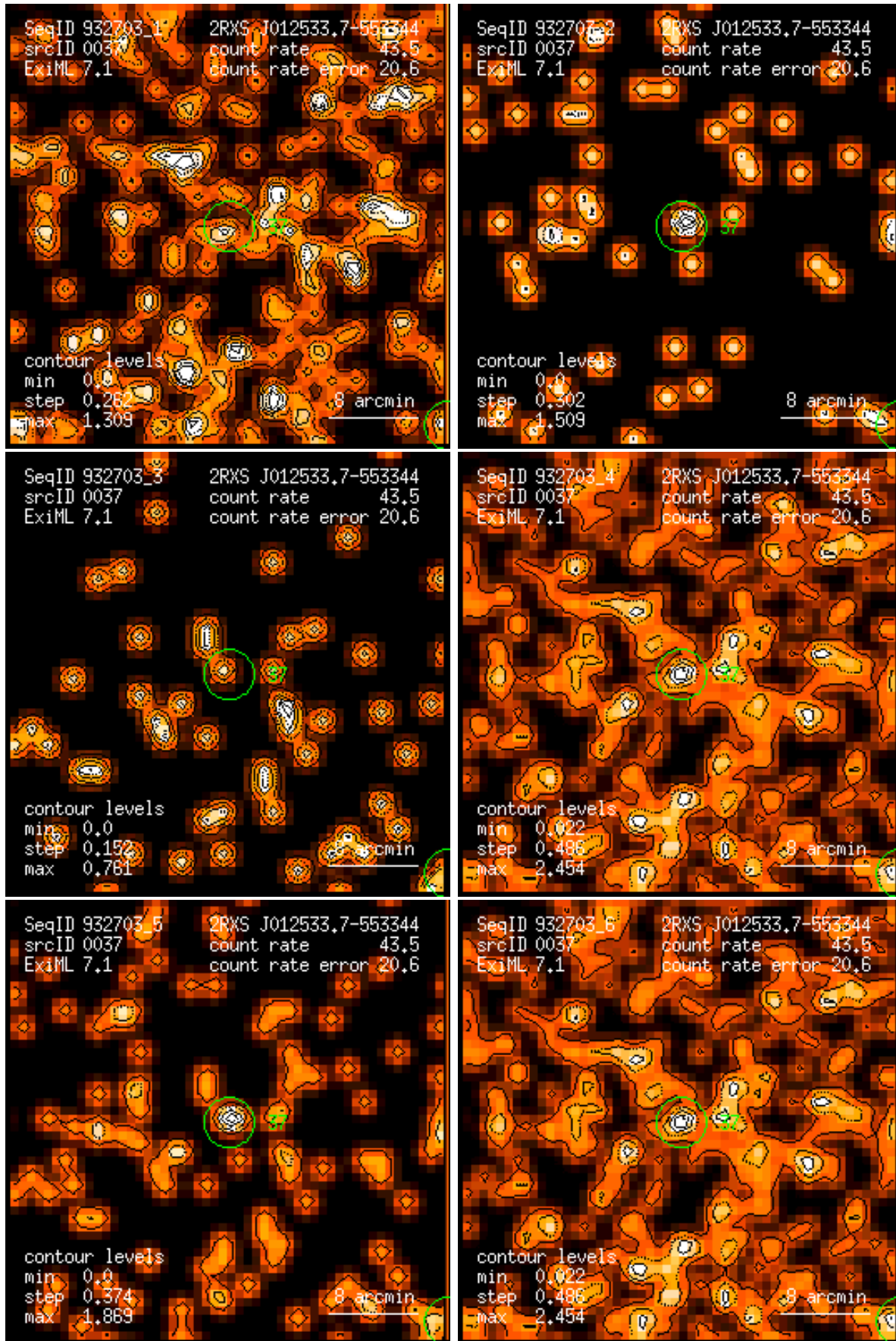
Figure 37: RASS 932703: detection 0037: band rate images, Gaussian filter: (1) PSPC channels 11 – 41, (2) 52 – 90, (3) 91 – 201, (4) 11 – 235, (5) 52 – 201, (6) 11 – 201. Broad band rates in counts/ks. Band rate contour levels in counts/ks/arcmin 2 .
